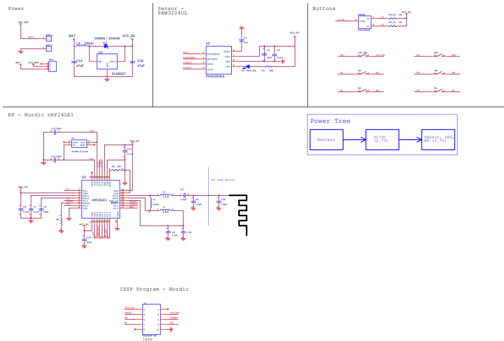
Figure 4. Application Circuit for 2.7V, one DC/DC (with Red LED)
