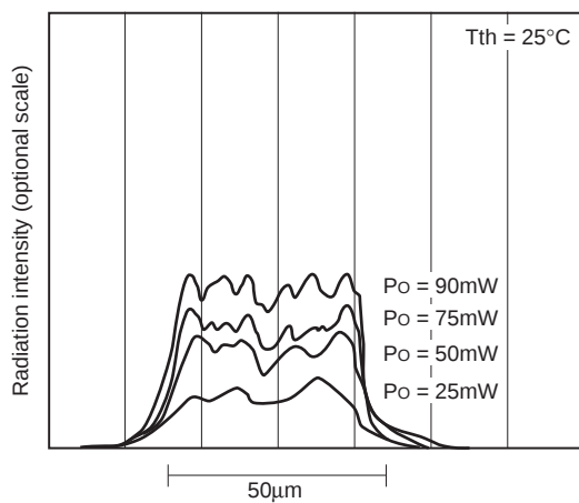
Power dependence of near field pattern
