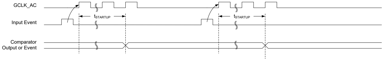
Figure 34-11. Single-Shot SleepWalking
