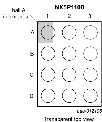
Fig 3. Pin configuration WLCSP12 package
