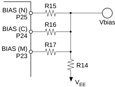
Figure 11 External Components of Bias Block
