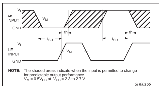
Waveform 3. Data set-up and hold times for the An input to the \overline{\text{LE}} input
