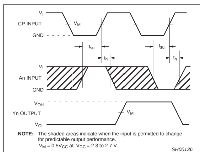
Waveform 5. Data set-up and hold times for the An input to the clock CP input
