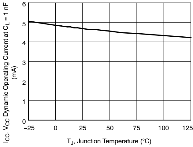
Figure 34. V_{CC} Dynamic Operating Current at C_L = 1.0 \text{ nF} vs. Junction Temperature
