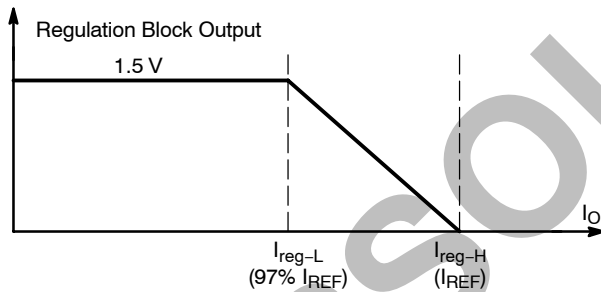
Figure 39. Regulation Characteristic
