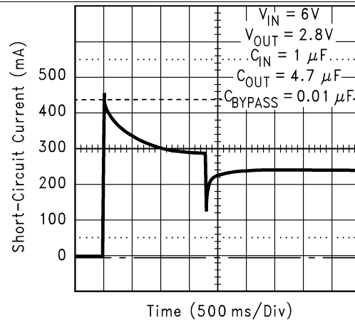
Figure 2. Short-Circuit Current
