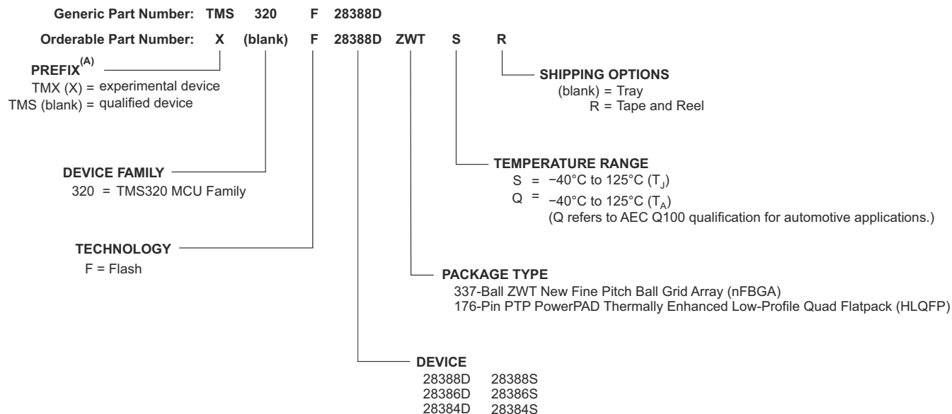
Figure 10-1. Device Nomenclature
