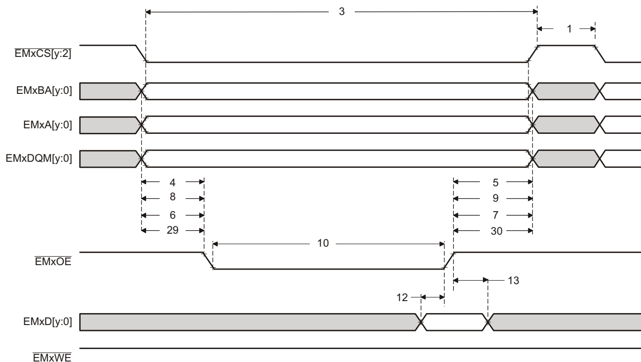
Figure 7-20. Asynchronous Memory Read Timing
