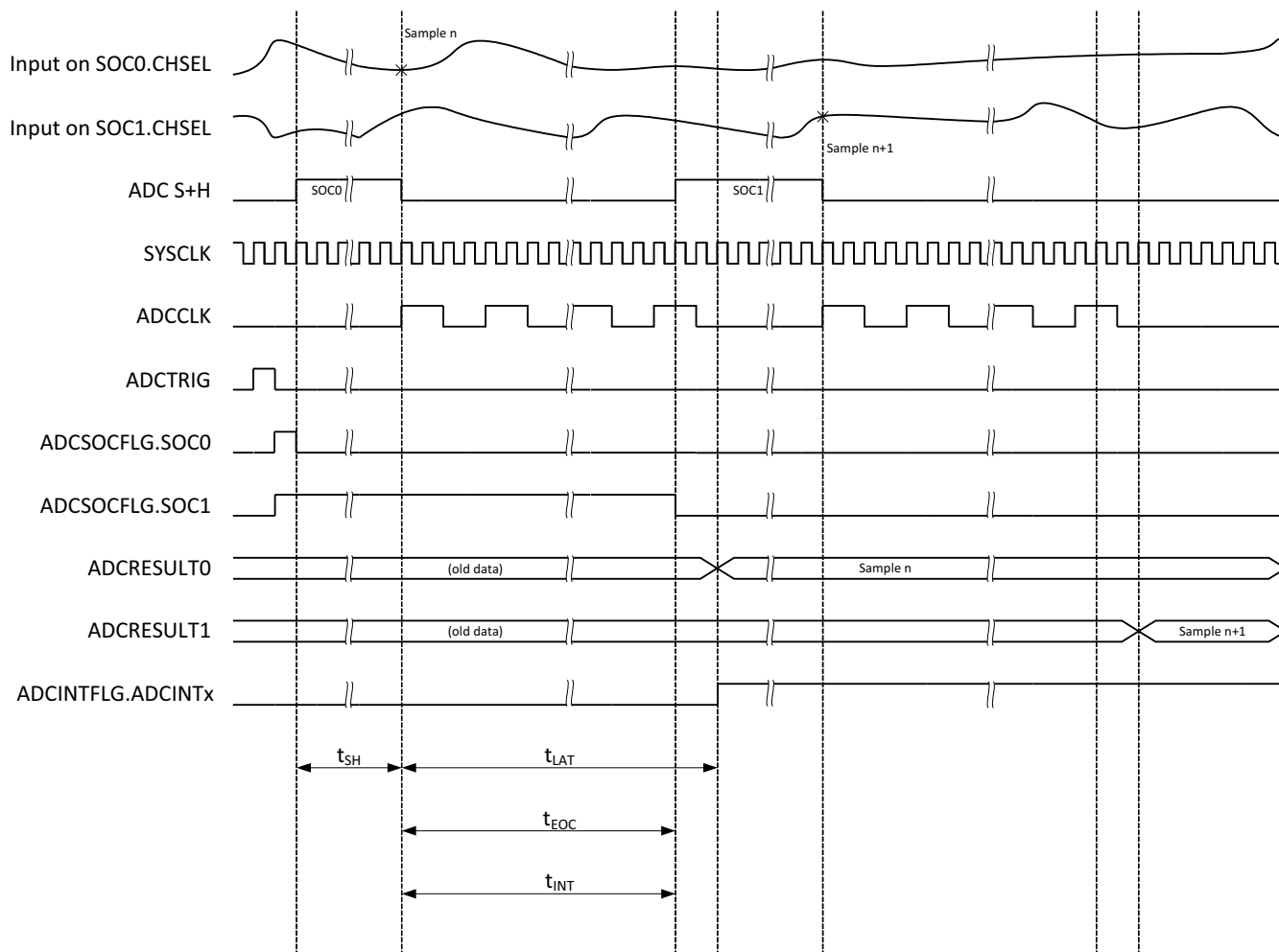
Figure 7-33. ADC Timings for 12-Bit Mode
