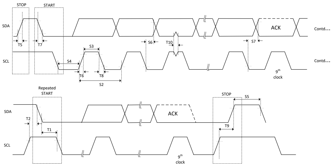
Figure 7-67. I2C Timing Diagram
