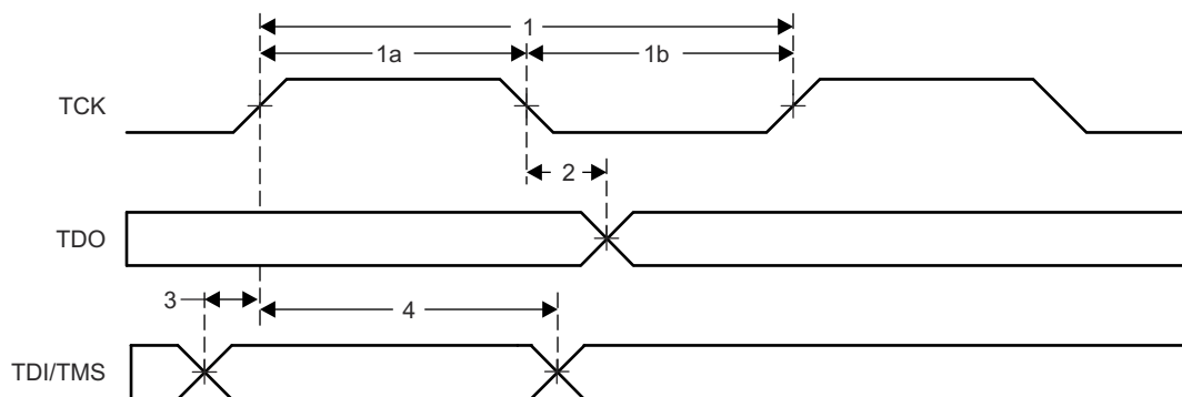
Figure 7-12. JTAG Timing
