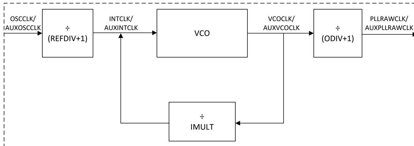
Figure 7-8. SYSPLL/AUXPLL
