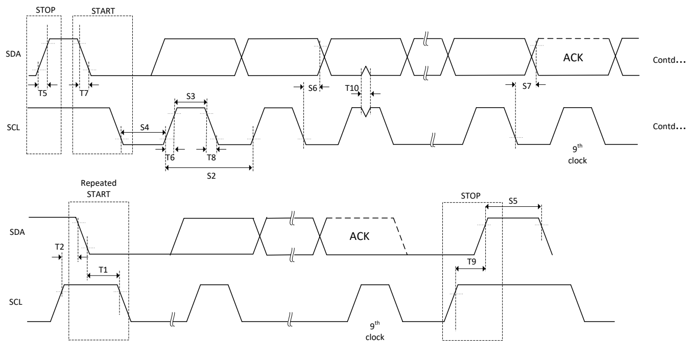
Figure 7-98. CM-I2C Timing Diagram
