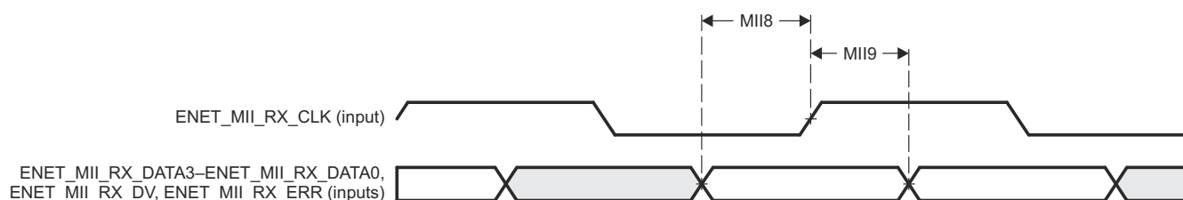
Figure 7-93. Receive Interface Timing (MII Operation)
