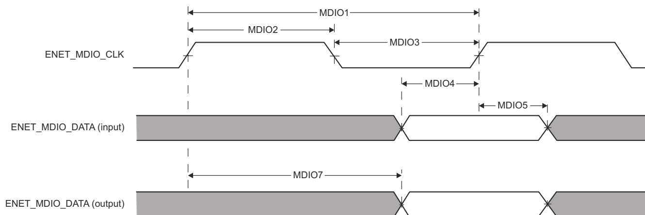
Figure 7-94. MDIO Timing Diagrams
