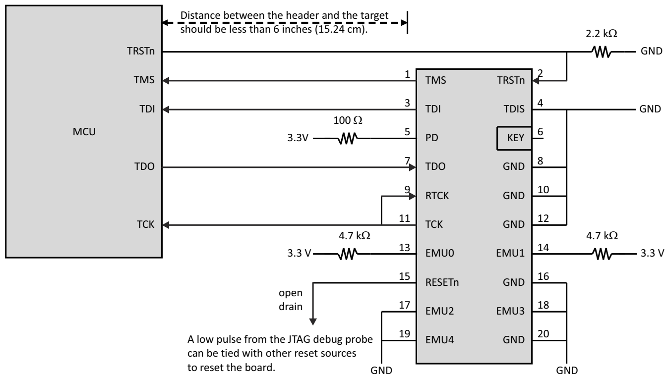
Figure 7-11. Connecting to the 20-Pin JTAG Header
