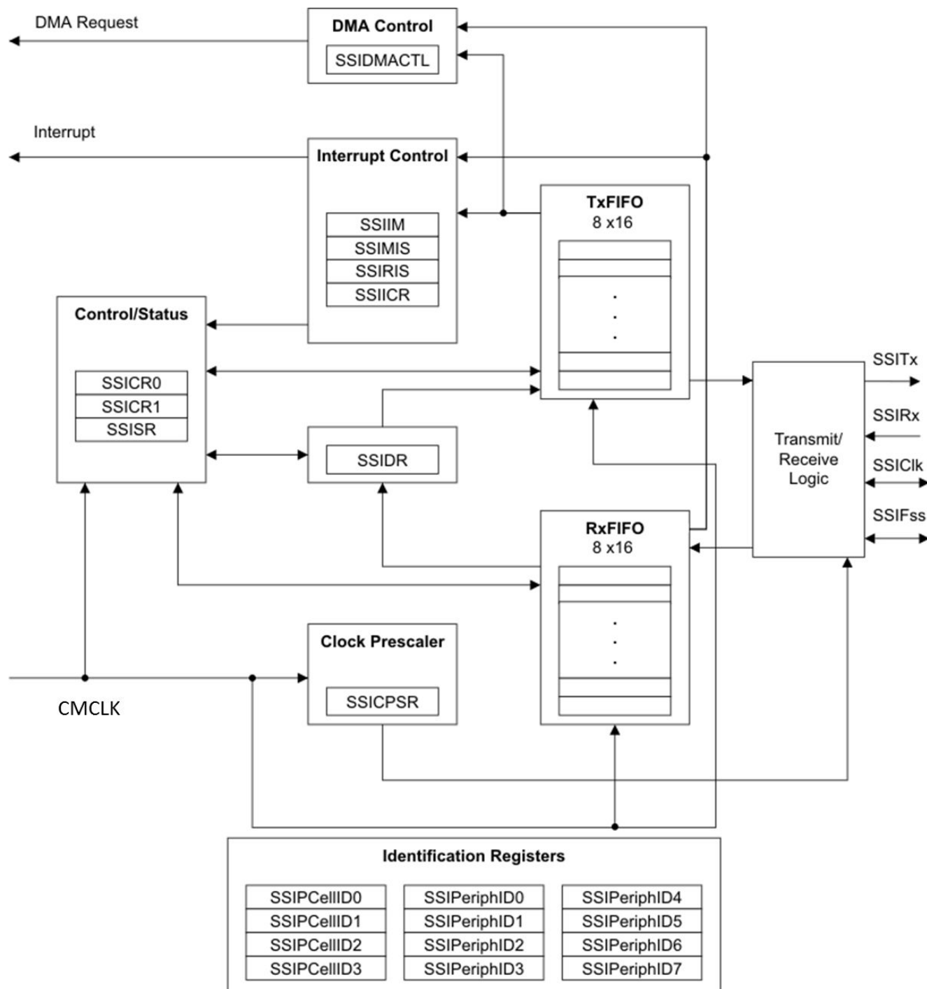
Figure 7-99. SSI Block Diagram
