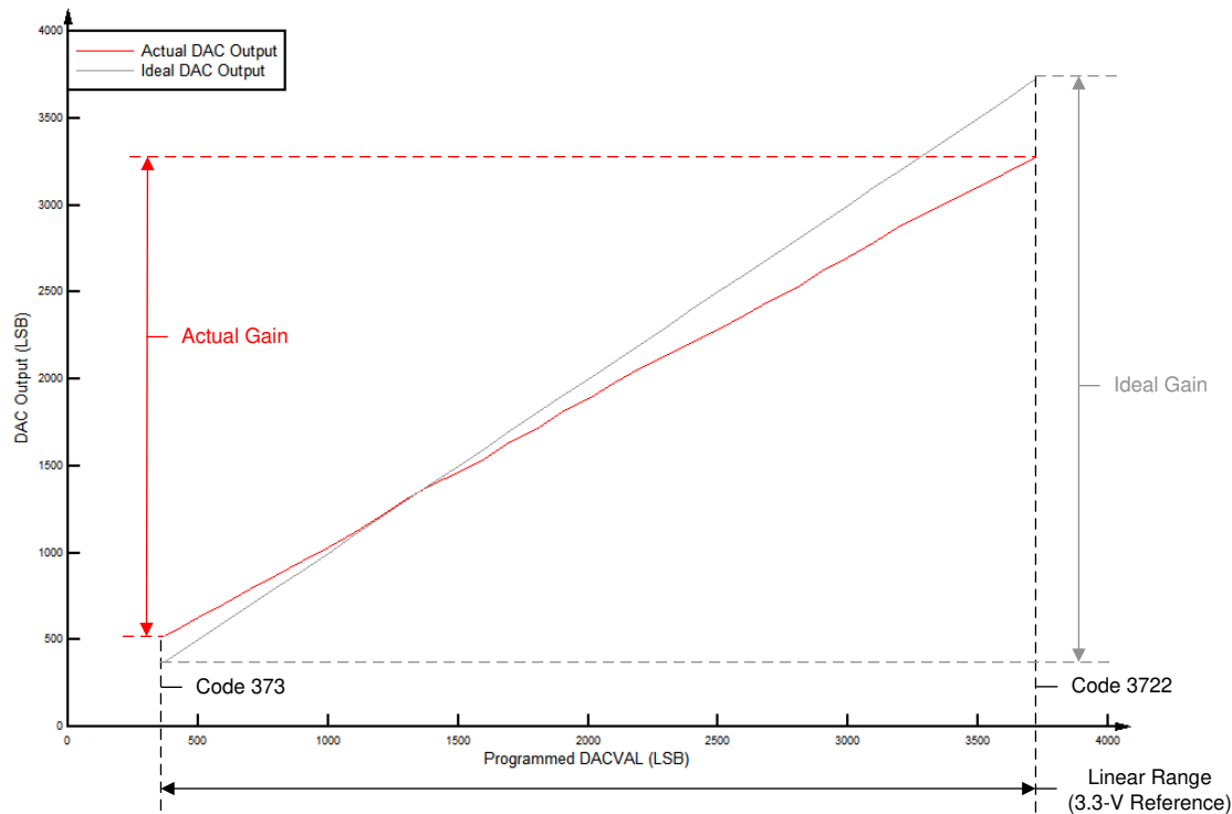
Figure 7-44. Buffered DAC Gain
