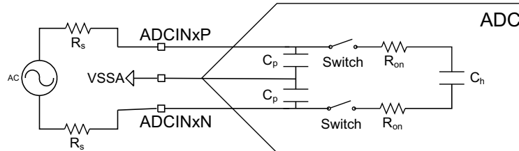
Figure 7-32. Differential Input Model
