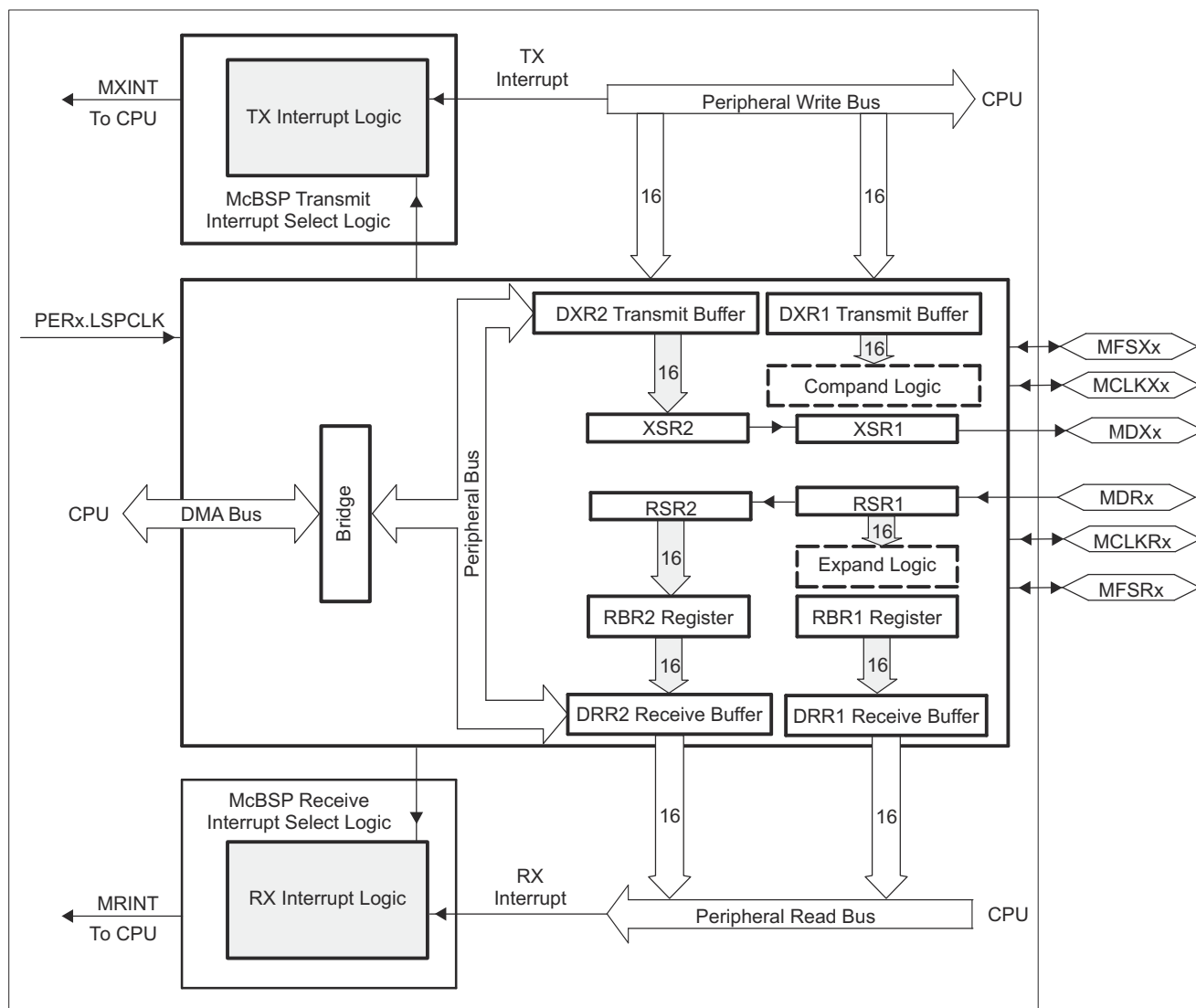
Figure 7-68. McBSP Block Diagram
