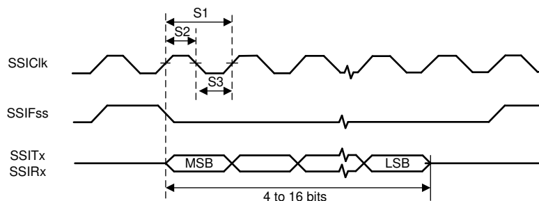
Figure 7-100. SSI Timing for TI Frame Format (FRF = 01), Single Transfer Timing Measurement
