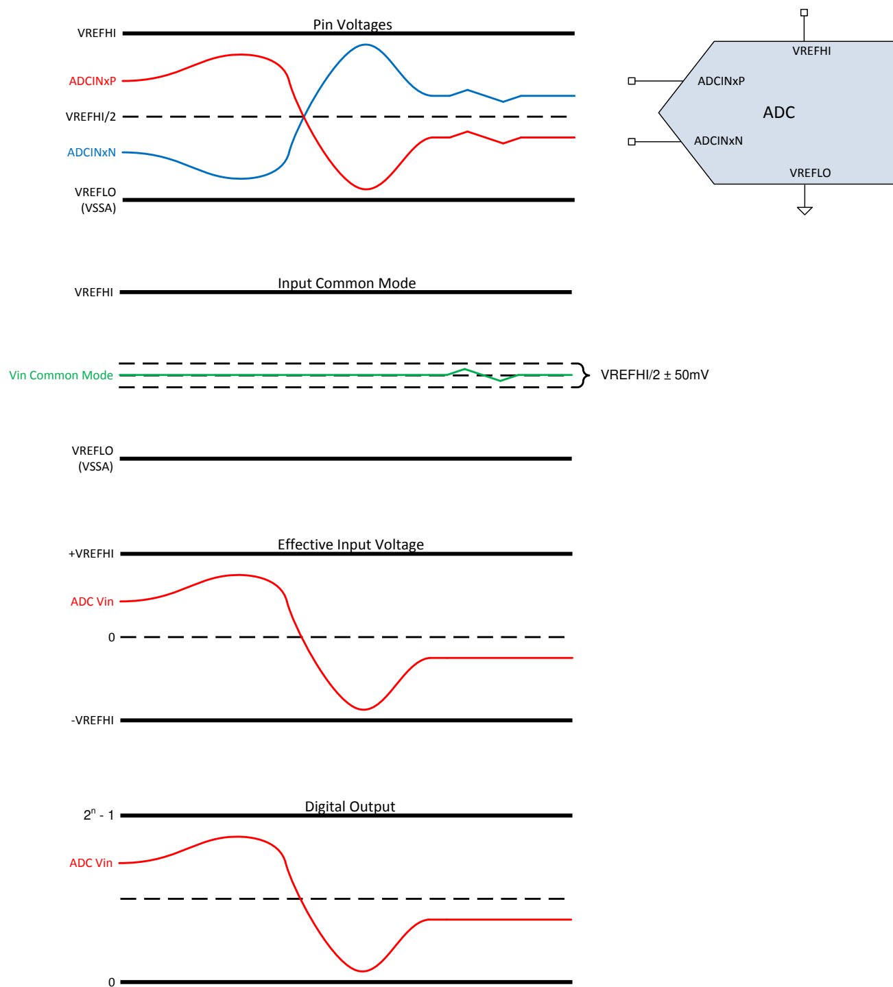
Figure 7-29. Differential Signaling Mode
