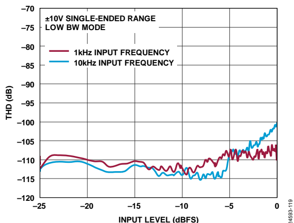
Figure 28. THD vs. Input Level, \pm 10 V Single-Ended Range, Low Bandwidth Mode
