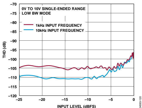
Figure 29. THD vs. Input Level, 0 V to 10 V Single-Ended Range, Low Bandwidth Mode
