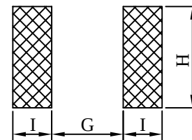
( PCB Pattern )
