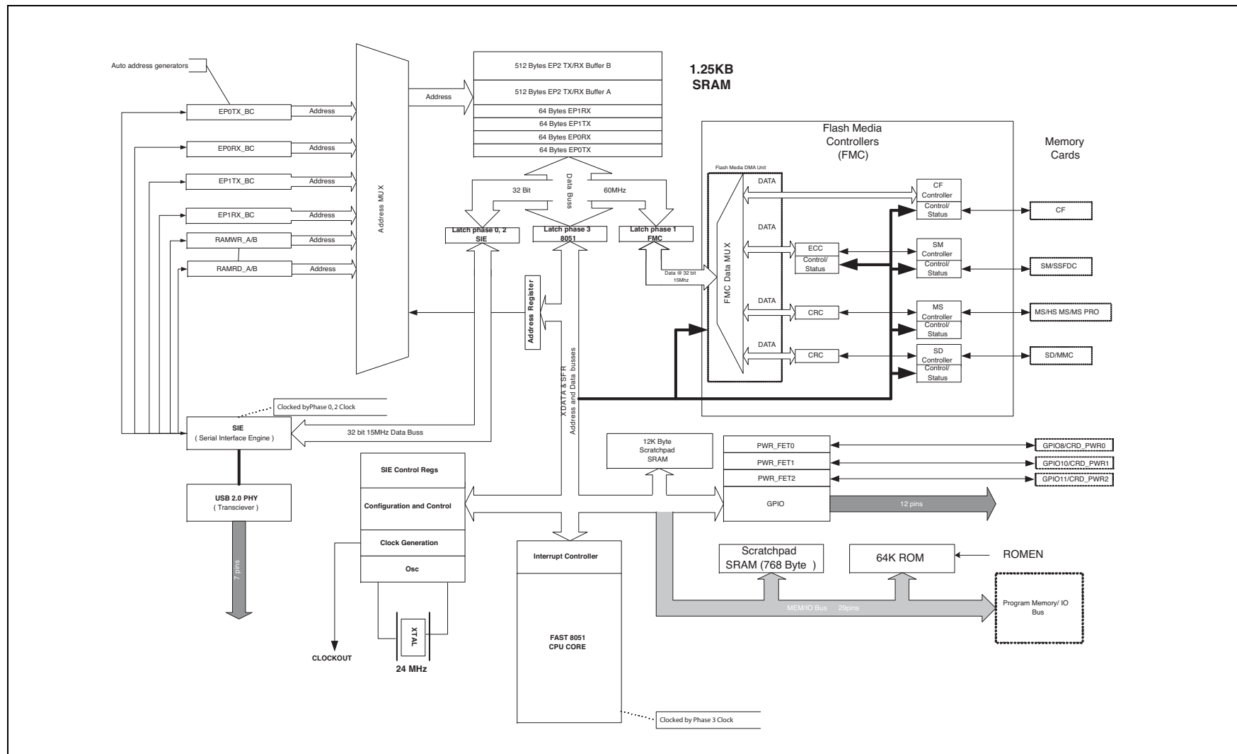
FIGURE 3-1: USB2227/USB2228 BLOCK DIAGRAM
