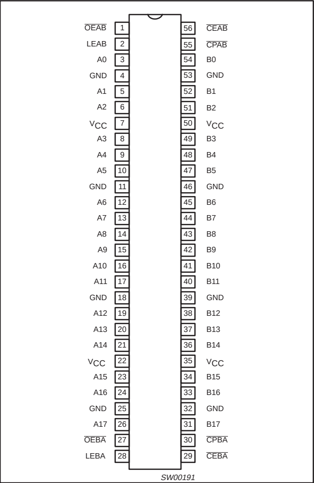
PIN CONFIGURATION
