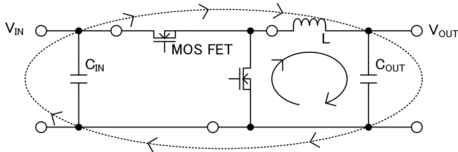
Figure 78. Current loop of buck converter
