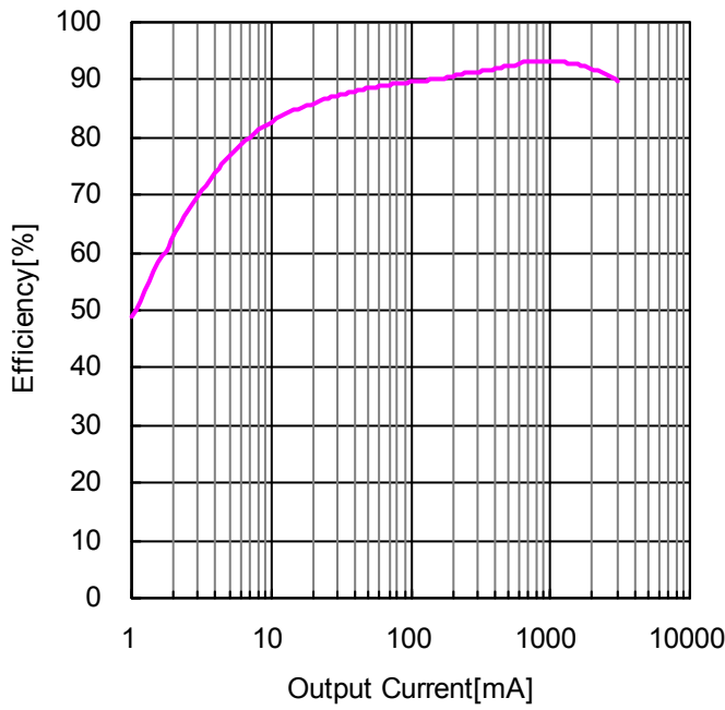
Figure 39. Efficiency - Output Current ( V_{IN}=12V , V_{OUT} = 5.0V , R3=10k\Omega )
