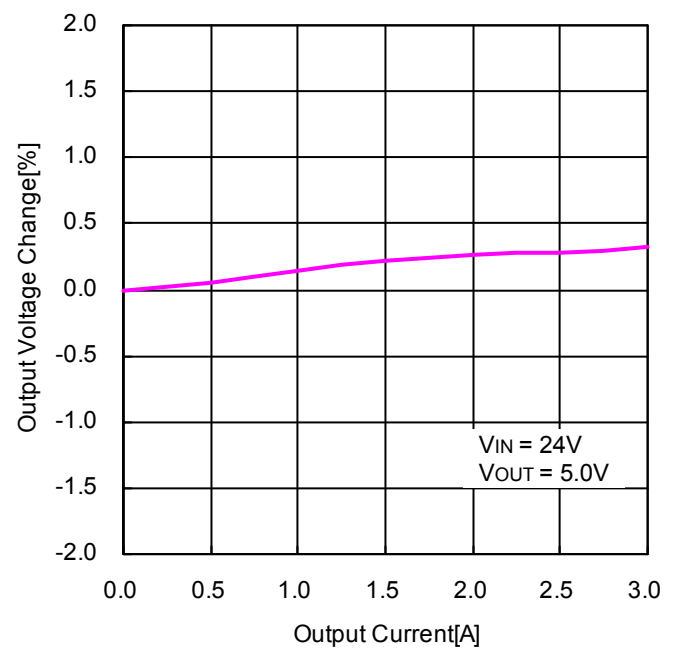
Figure 31. VOUT Load Regulation (VOUT = 5V)
