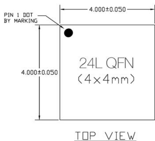
Figure 19. Package Drawing
