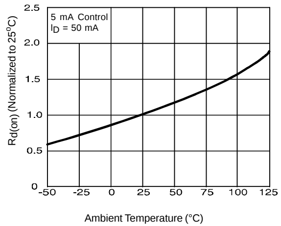
Figure 2. Typical On-Resistance
