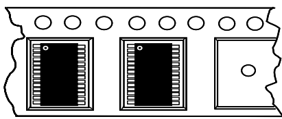
Typical SSOP, TSSOP Package Orientation
