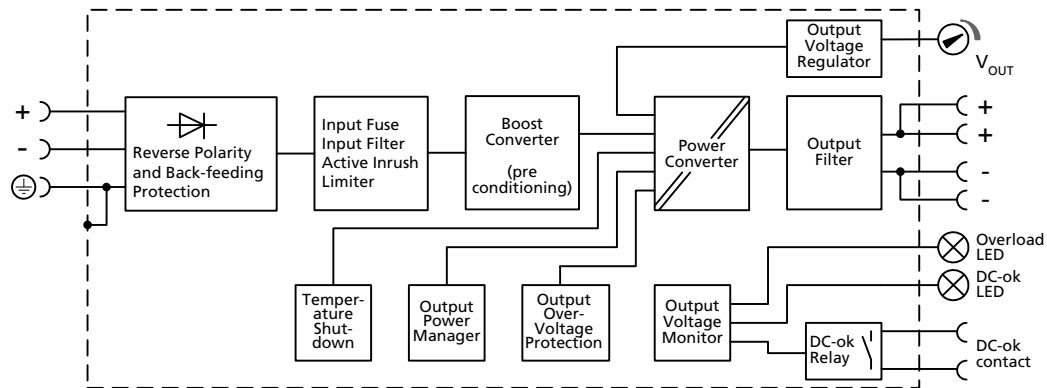
Fig. 11-1 Functional diagram
