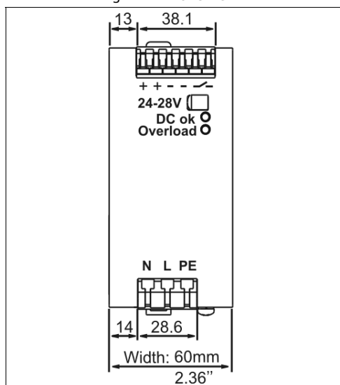
Fig. 21-1 Front view
