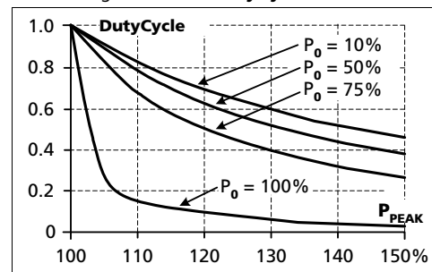
Fig. 23-2 Max. duty cycle curve
