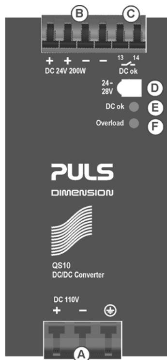
Fig. 13-1 Front side
