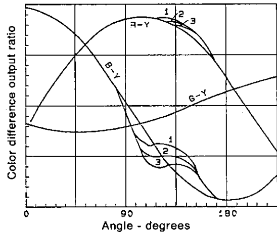
Flesh-tone center adjustment
