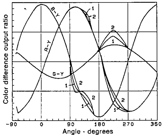
Flesh-tone correction and green enhancement characteristics
