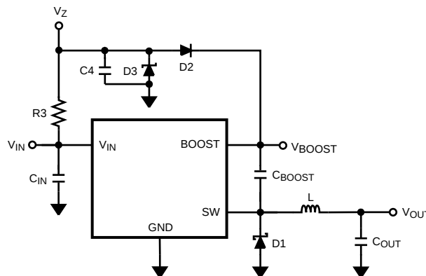
Figure 23. Boost Voltage Supplied from the Shunt Zener on V IN
