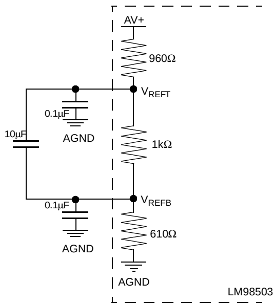
Figure 16: Reference Bypassing
