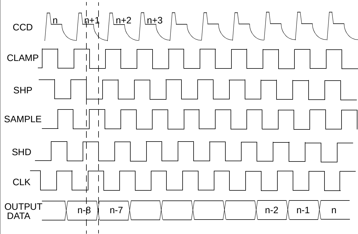
Figure 8: System Timing
