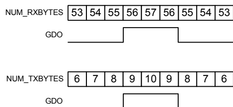
Figure 20: FIFO_THR=13 vs. Number of Bytes in FIFO ( GDOx_CFG=0x00 in RX and GDOx_CFG=0x02 in TX)
