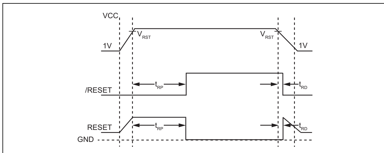
FIGURE 1-1: Timing Diagram.
