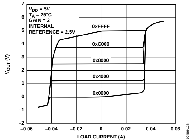
Figure 32. Source and Sink Capability at 5 V
