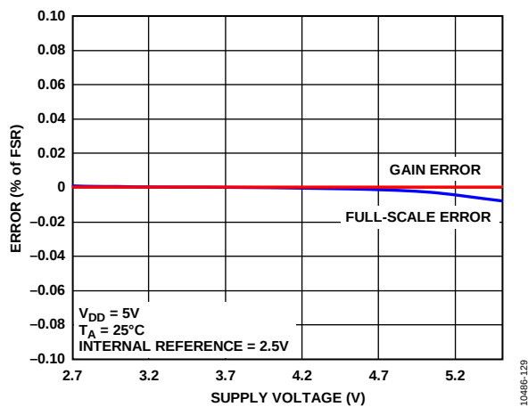
Figure 24. Gain Error and Full-Scale Error vs. Supply
