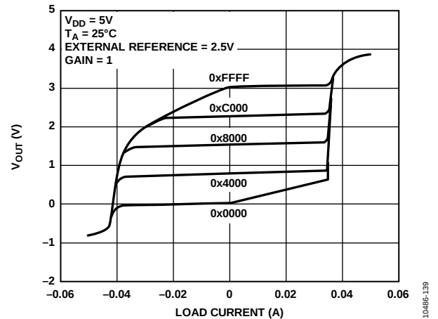
Figure 33. Source and Sink Capability at 3 V
