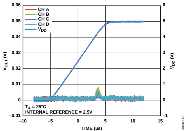
Figure 36. Power-On Reset to 0 V
