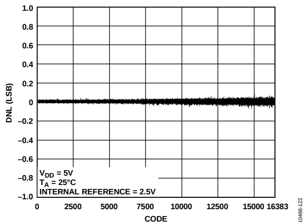
Figure 17. AD5695R DNL
