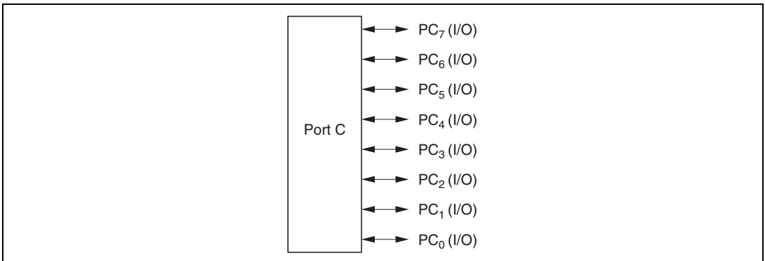
Figure 8.18 Port C Pin Functions (Modes 3 and 7)
