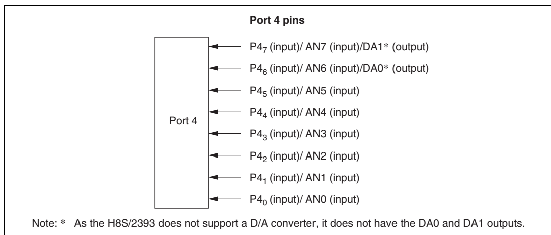
Figure 8.4 Port 4 Pin Functions
