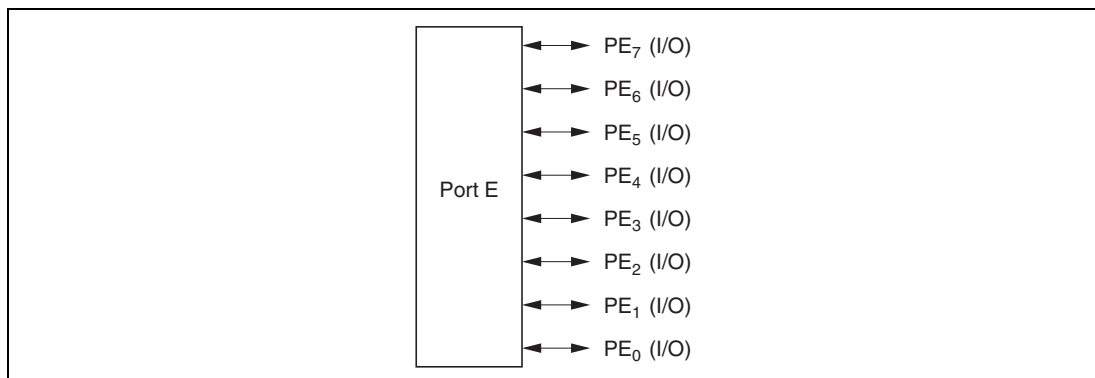
Figure 8.24 Port E Pin Functions (Modes 3 and 7)
