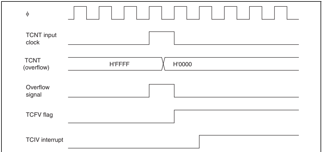
Figure 9.44 TCIV Interrupt Setting Timing
