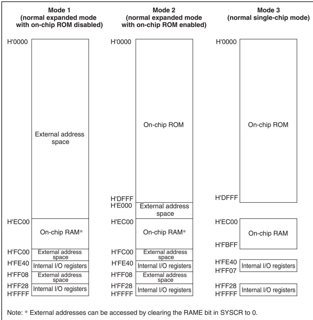
Figure 3.1 Memory Map in Each Operating Mode in the H8S/2355
