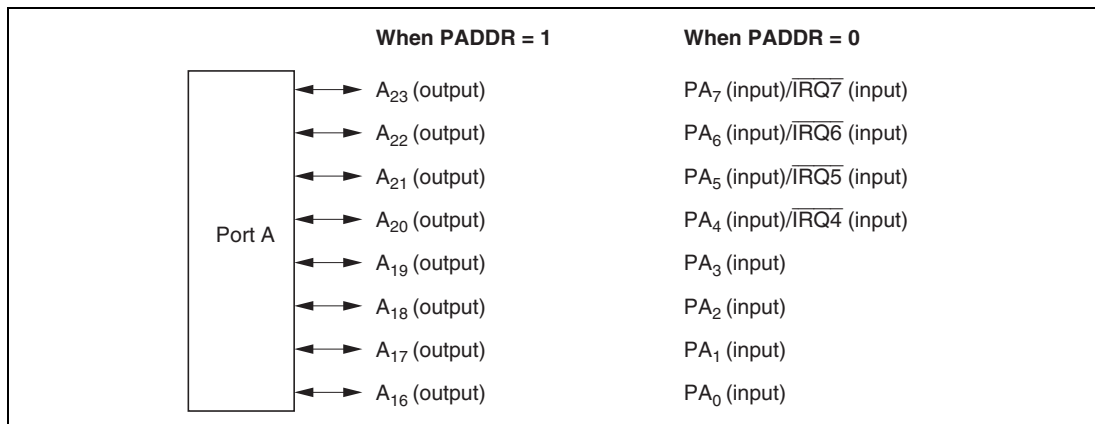
Figure 8.10 Port A Pin Functions (Mode 6)
