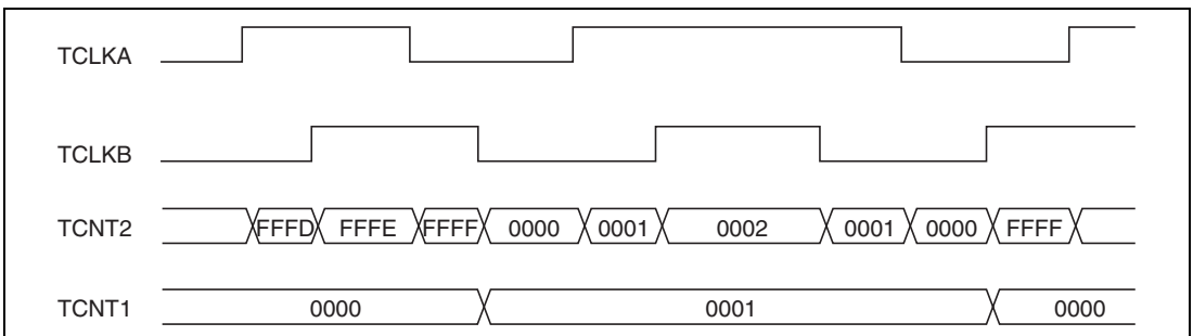
Figure 9.23 Example of Cascaded Operation (2)
