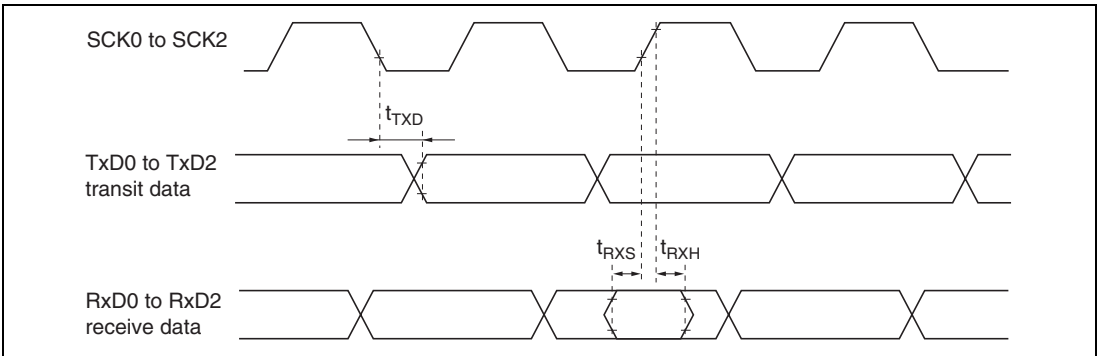
Figure 20.22 SCI Input/Output Timing (Clock Synchronous Mode)
