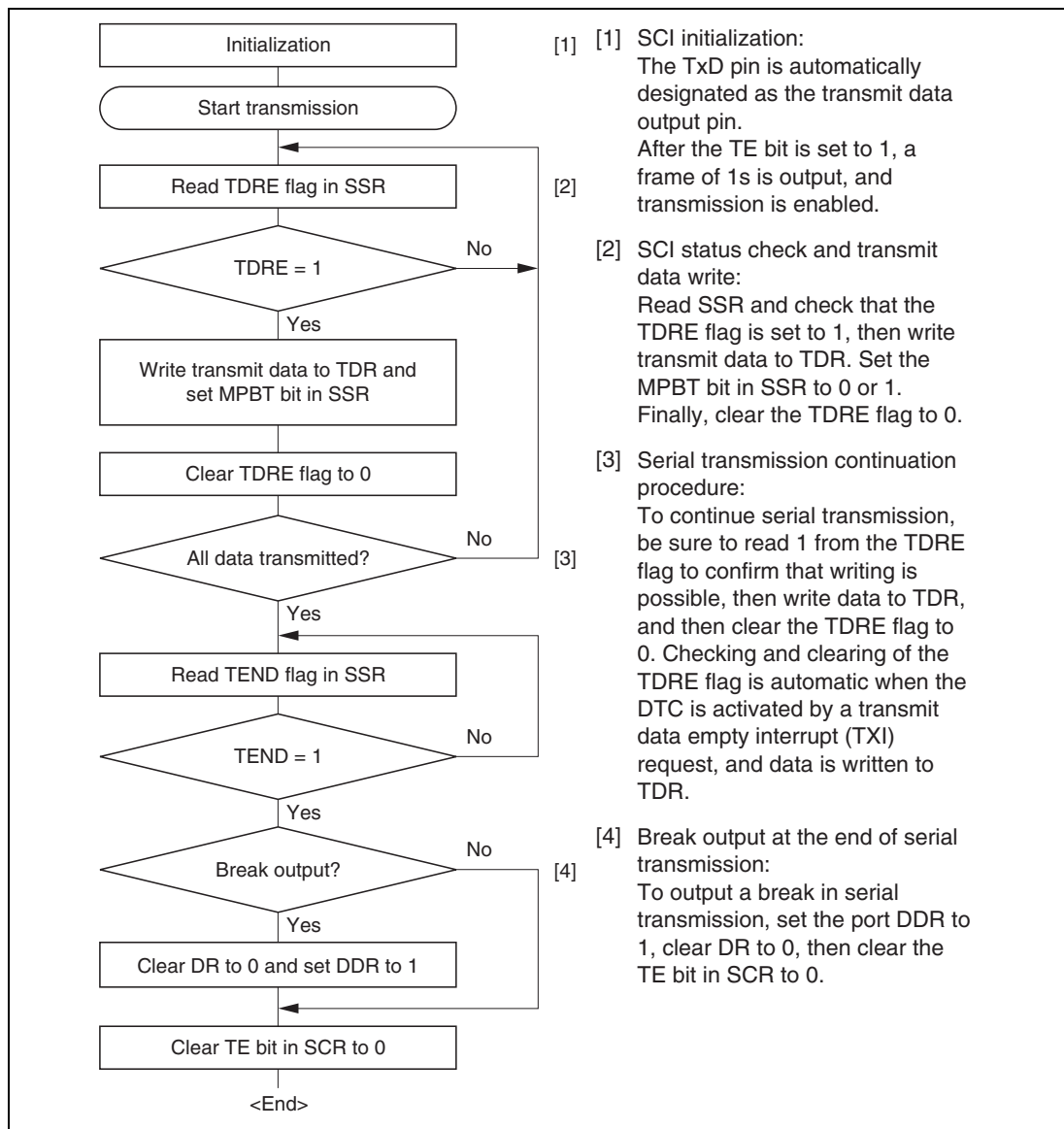
Figure 12.10 Sample Multiprocessor Serial Transmission Flowchart
