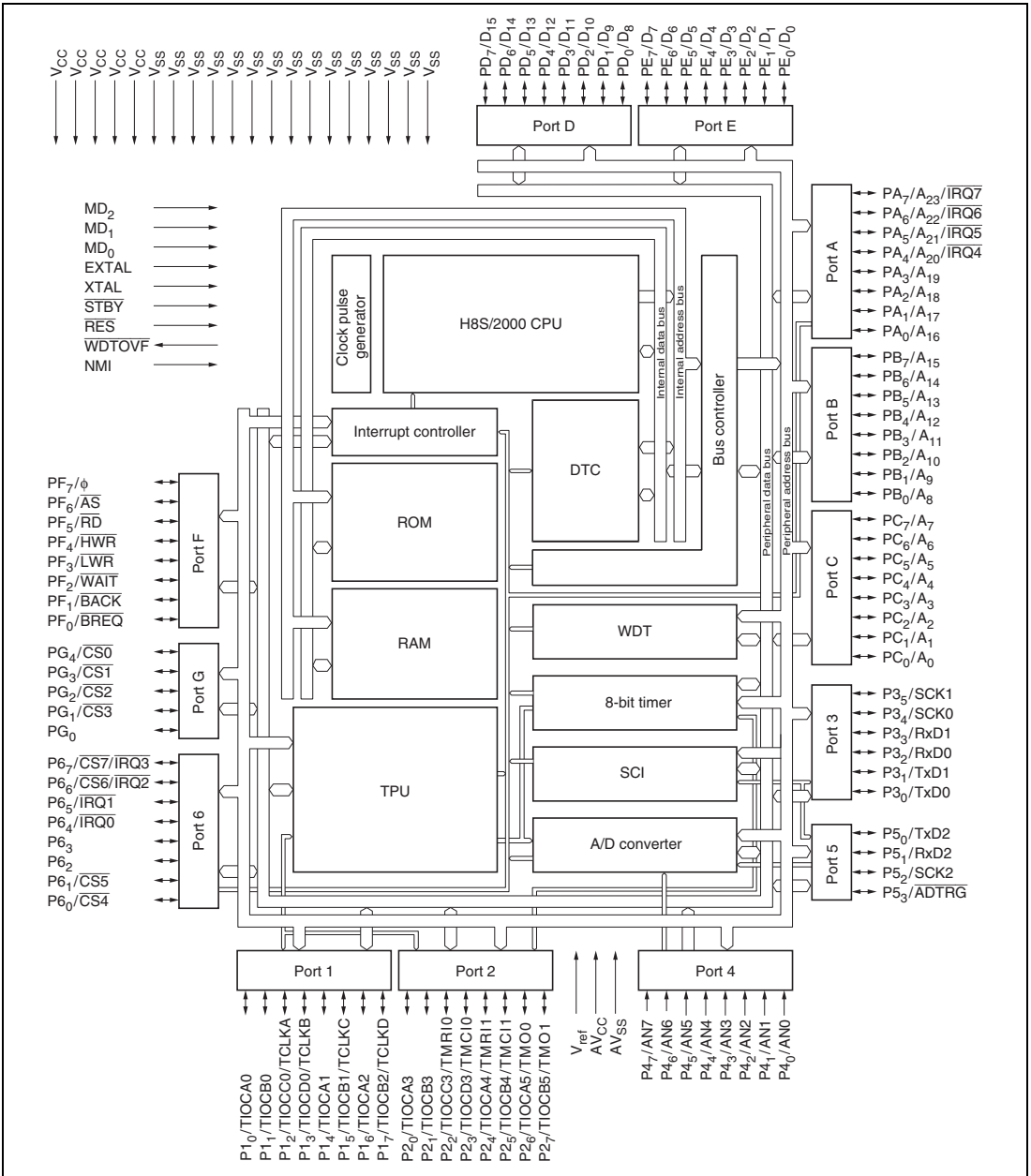
Figure 1.2 Block Diagram (H8S/2393)
