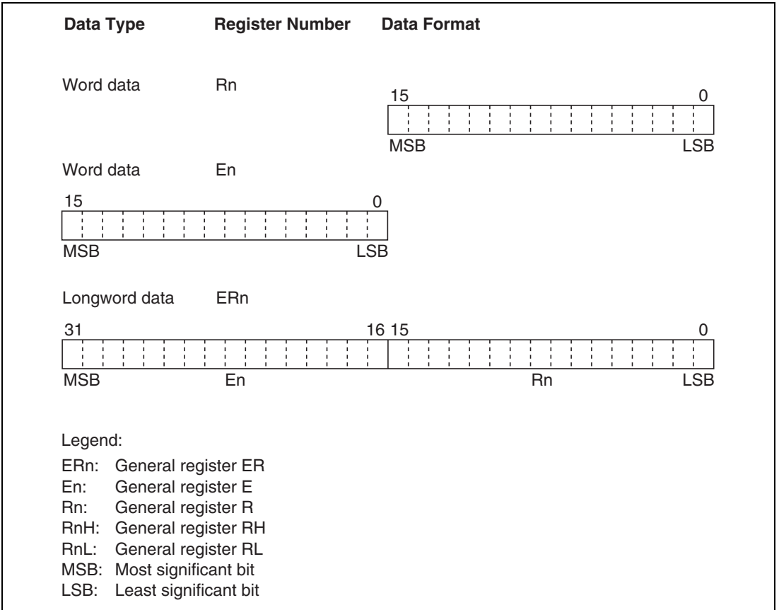
Figure 2.10 General Register Data Formats (cont)
