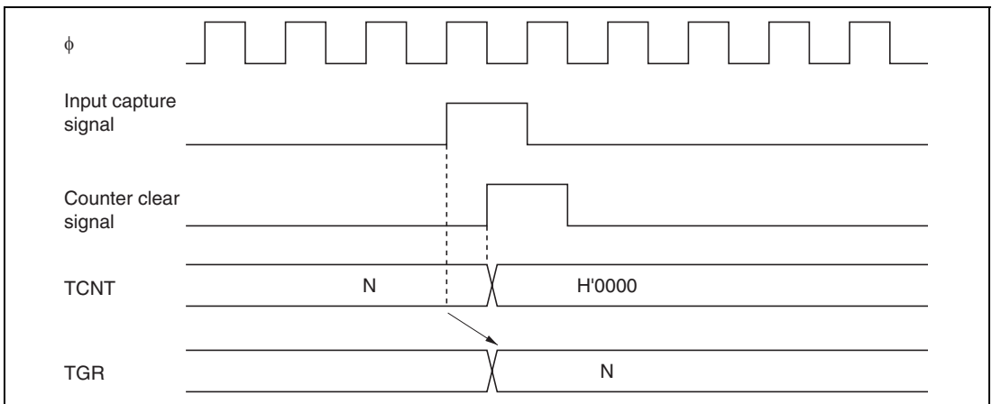
Figure 9.39 Counter Clear Timing (Input Capture)
