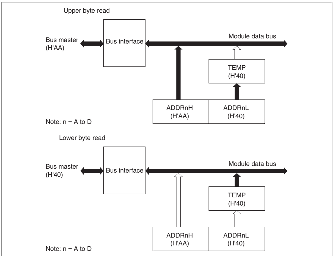
Figure 14.2 ADDR Access Operation (Reading H'AA40)
