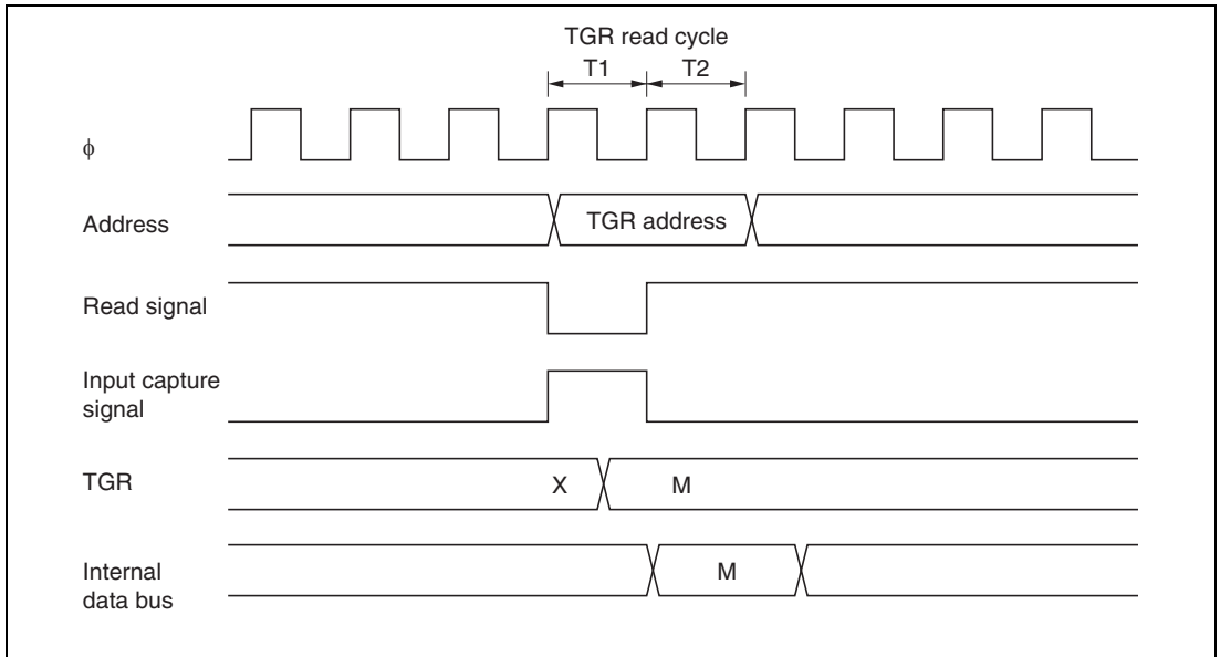
Figure 9.53 Contention between TGR Read and Input Capture
