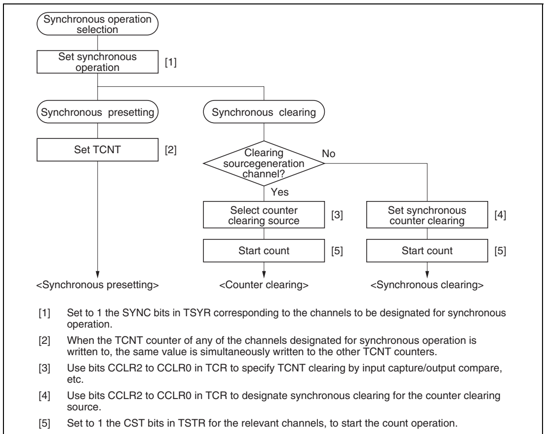
Figure 9.14 Example of Synchronous Operation Setting Procedure
