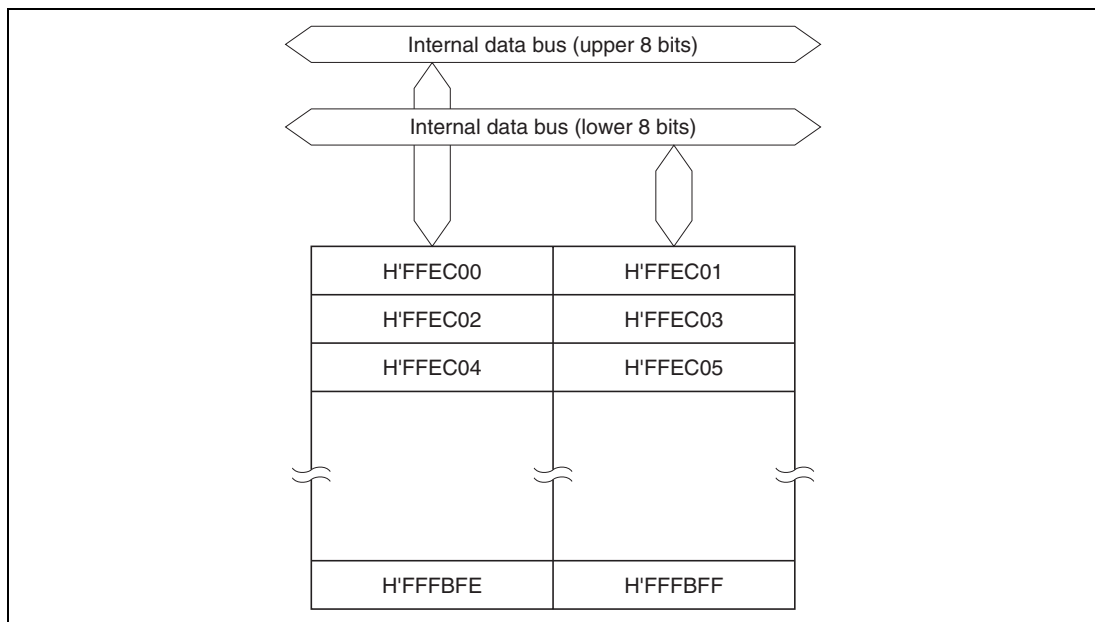
Figure 16.1 Block Diagram of RAM (H8S/2355)
