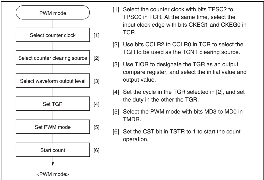
Figure 9.24 Example of PWM Mode Setting Procedure
