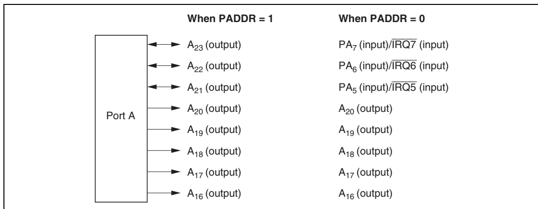
Figure 8.9 Port A Pin Functions (Modes 4 and 5)
