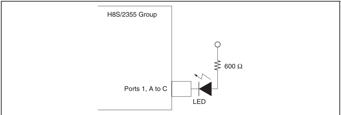
Figure 20.2 LED Drive Circuit (Example)
