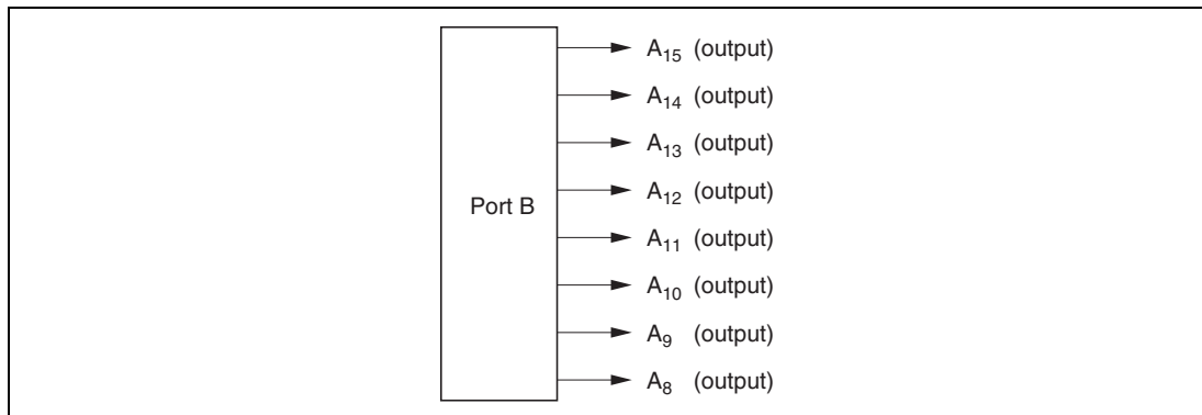
Figure 8.12 Port B Pin Functions (Modes 1, 4, and 5)
