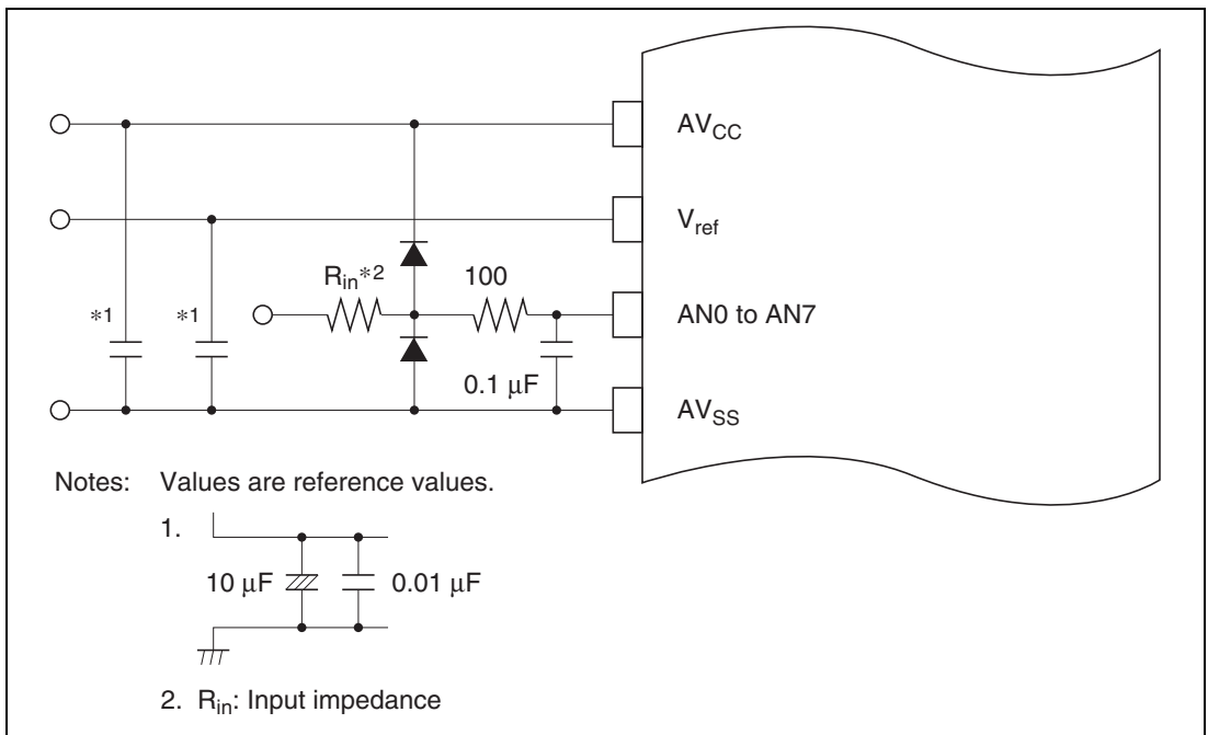
Figure 14.7 Example of Analog Input Protection Circuit
