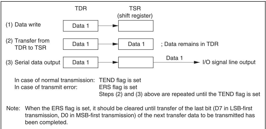
Figure 13.5 Relation Between Transmit Operation and Internal Registers
