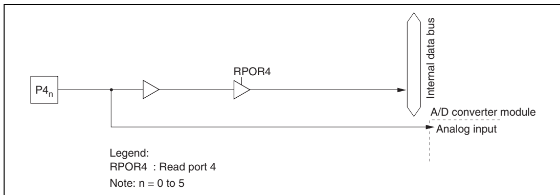
Figure C.4 (a) Port 4 Block Diagram (Pins P4 0 to P4 5 in H8S/2355 and H8S/2353, Pins P4 0 to P4 7 in H8S/2393)
