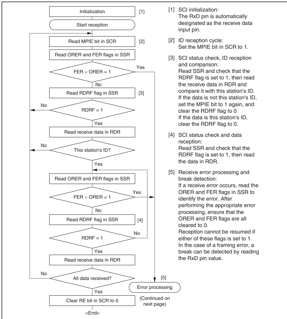
Figure 12.12 Sample Multiprocessor Serial Reception Flowchart
