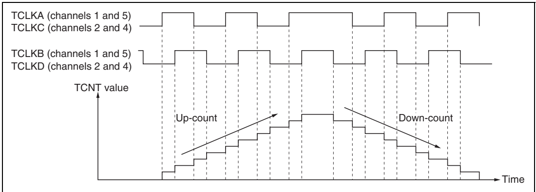
Figure 9.29 Example of Phase Counting Mode 1 Operation
