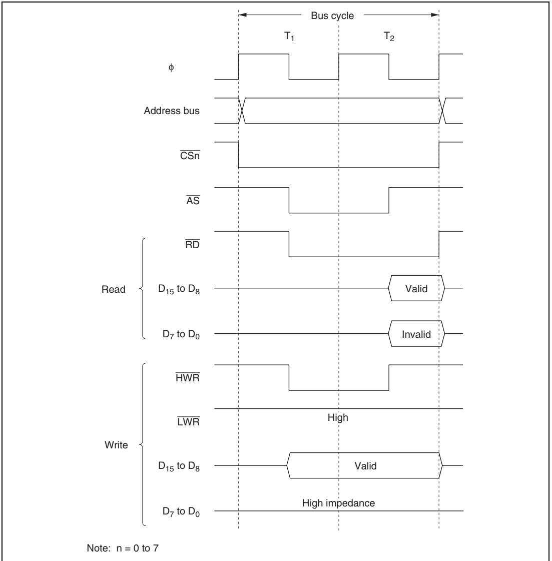
Figure 6.6 Bus Timing for 8-Bit 2-State Access Space
