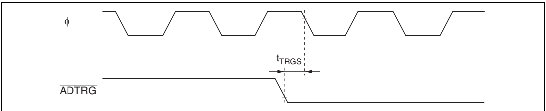
Figure 20.23 A/D Converter External Trigger Input Timing
