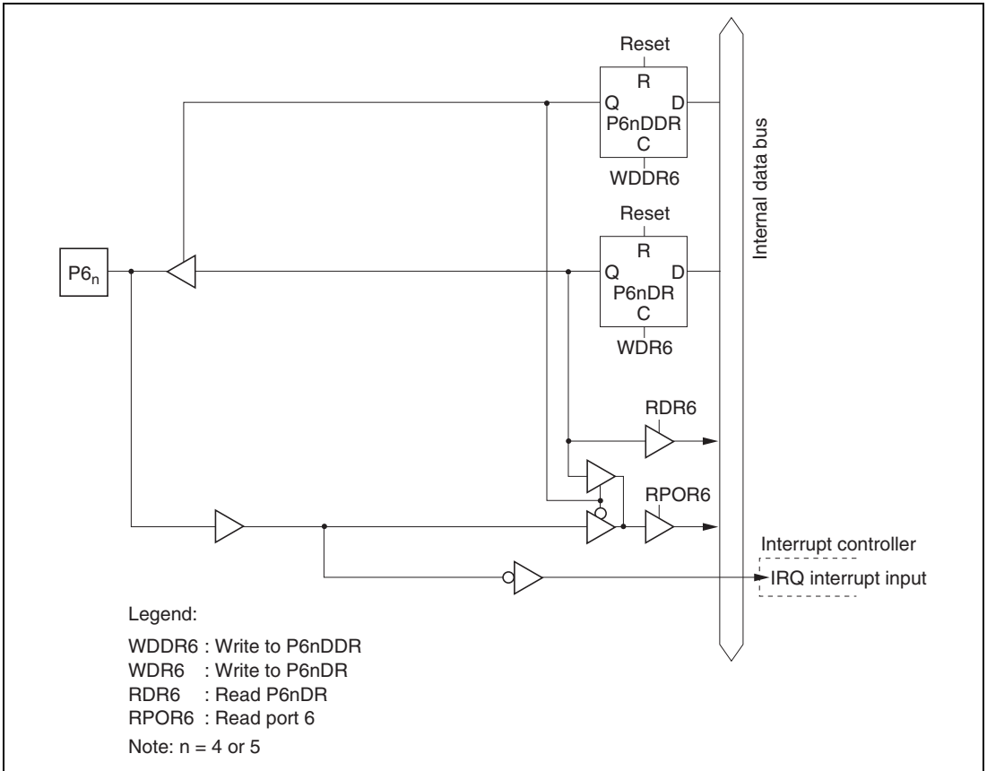
Figure C.6 (c) Port 6 Block Diagram (Pins P6 n and P6 n )
