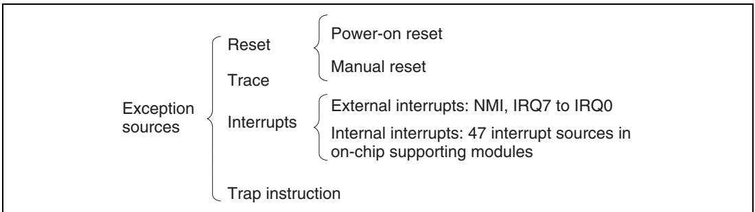
Figure 4.1 Exception Sources
