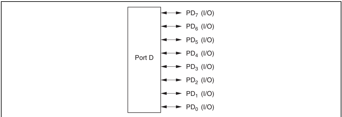
Figure 8.21 Port D Pin Functions (Modes 3 and 7)
