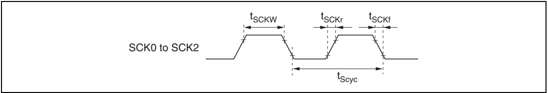
Figure 20.21 SCK Clock Input Timing
