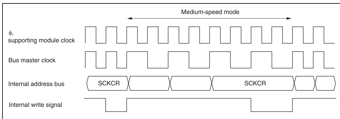
Figure 19.1 Medium-Speed Mode Transition and Clearance Timing
