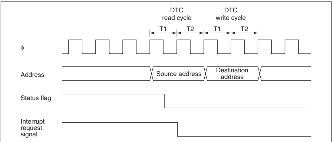
Figure 9.47 Timing for Status Flag Clearing by DTC Activation
