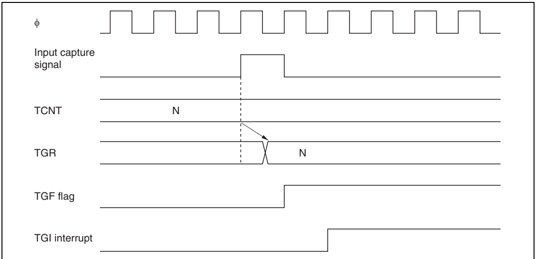
Figure 9.43 TGI Interrupt Timing (Input Capture)
