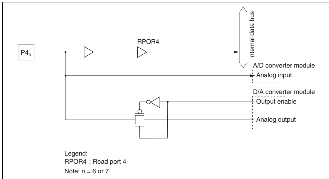
Figure C.4 (b) Port 4 Block Diagram (Pins P4 6 and P4 7 in H8S/2355 and H8S/2353)
