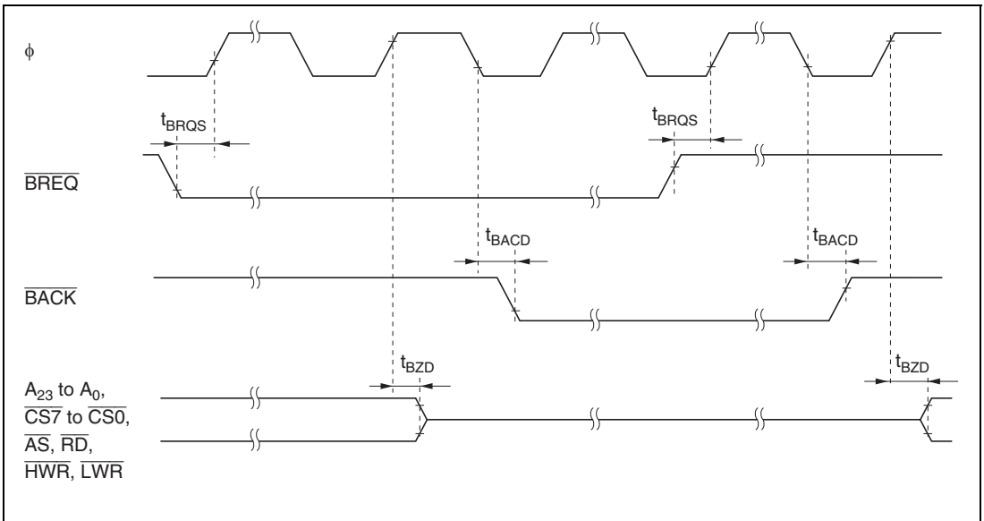
Figure 20.13 External Bus Release Timing
