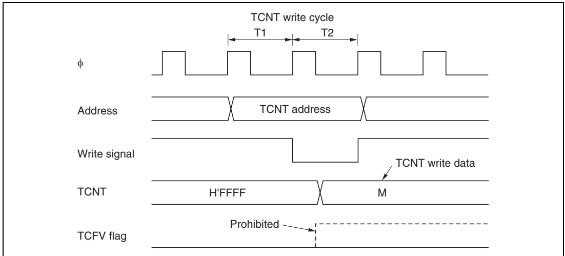
Figure 9.57 Contention between TCNT Write and Overflow
