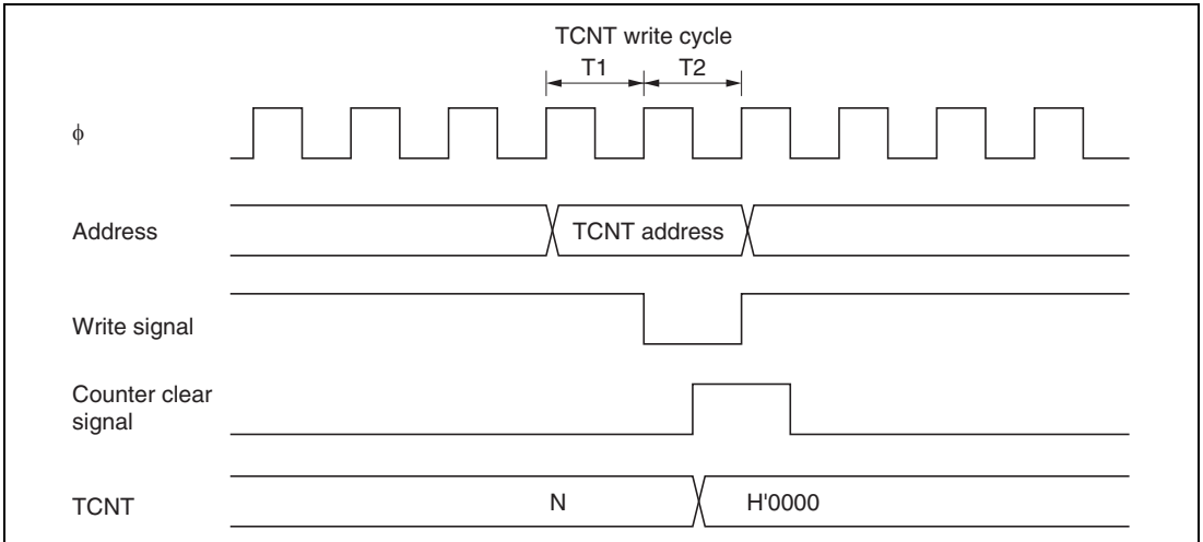
Figure 9.49 Contention between TCNT Write and Clear Operations
