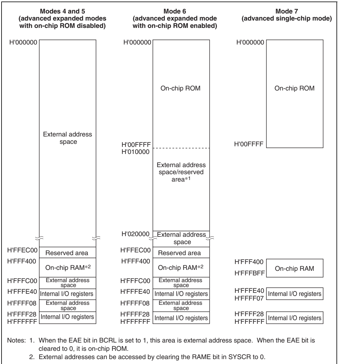
Figure 3.2 Memory Map in Each Operating Mode in the H8S/2353 (cont)
