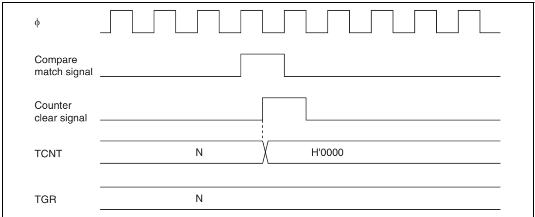
Figure 9.38 Counter Clear Timing (Compare Match)
