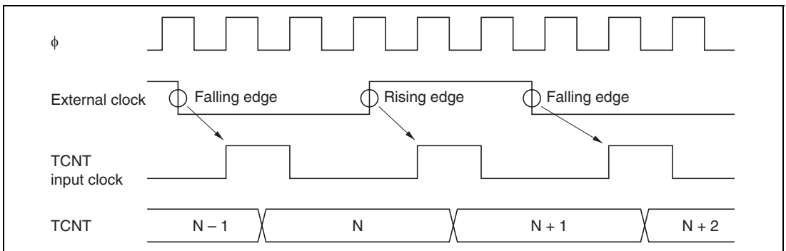
Figure 9.35 Count Timing in External Clock Operation
