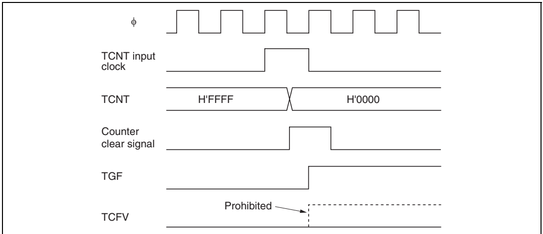
Figure 9.56 Contention between Overflow and Counter Clearing
