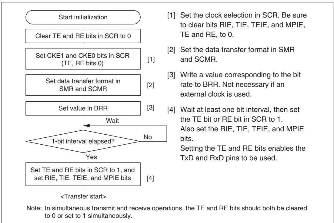
Figure 12.15 Sample SCI Initialization Flowchart
