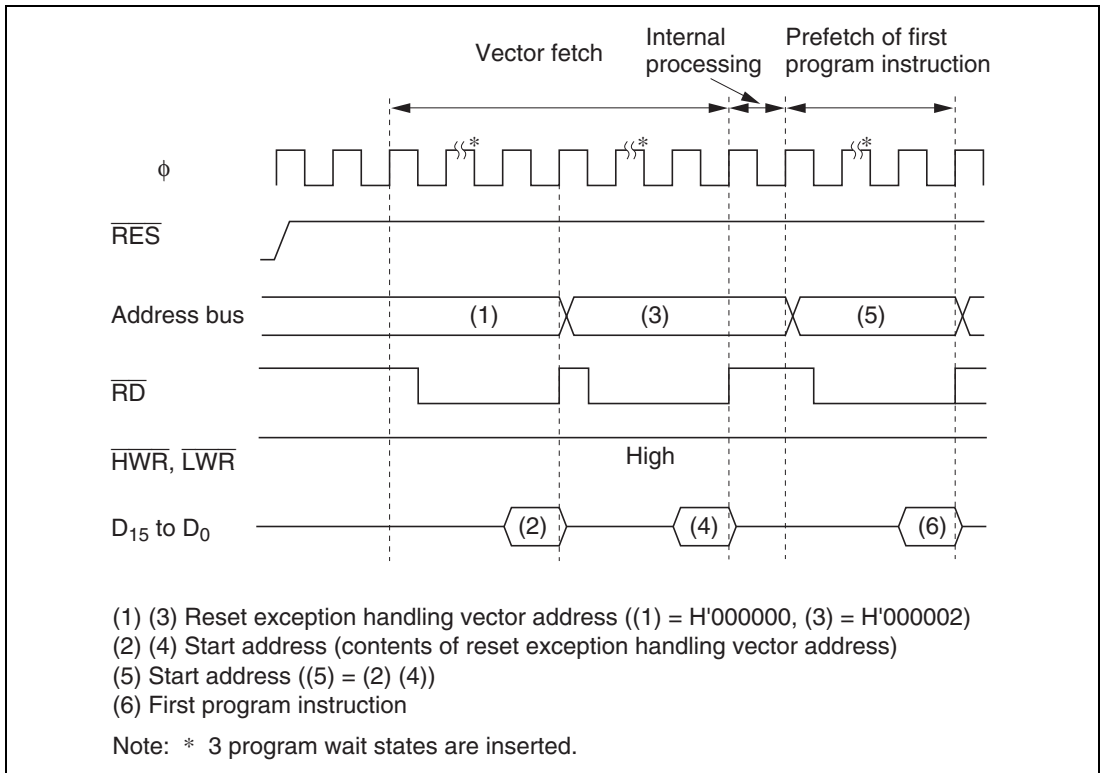
Figure 4.3 Reset Sequence (Mode 4)
