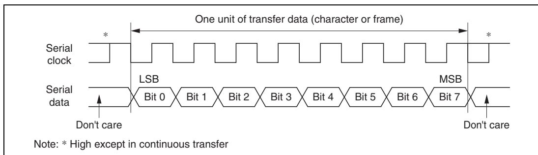
Figure 12.14 Data Format in Synchronous Communication
