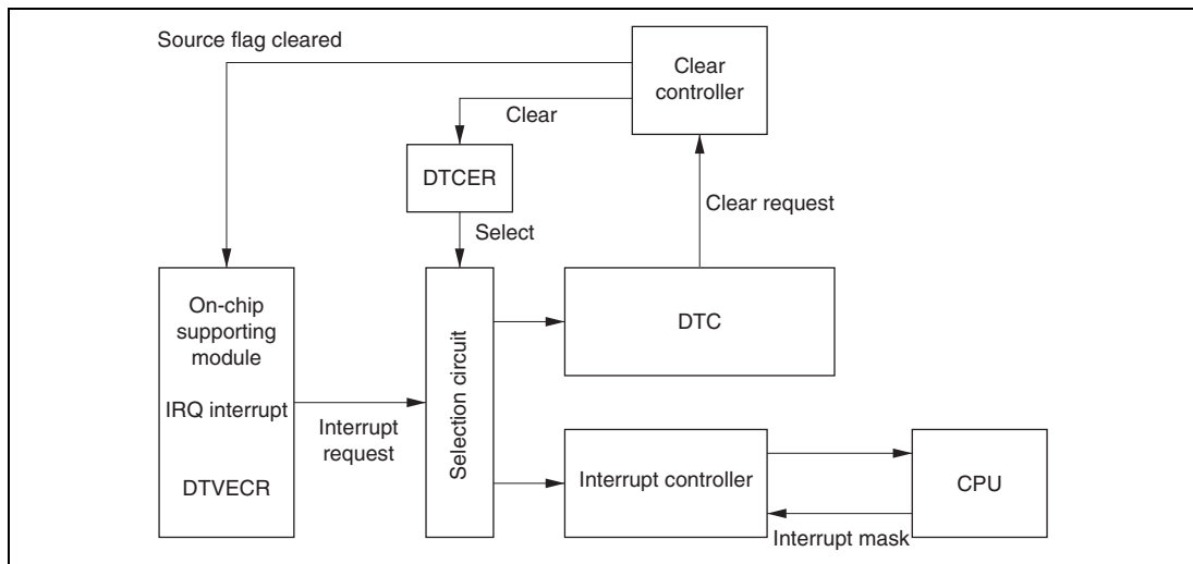
Figure 7.3 Block Diagram of DTC Activation Source Control
