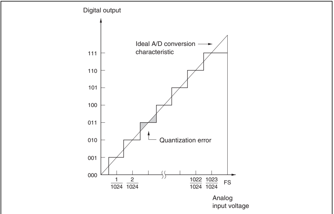
Figure 14.9 A/D Conversion Precision Definitions (1)
