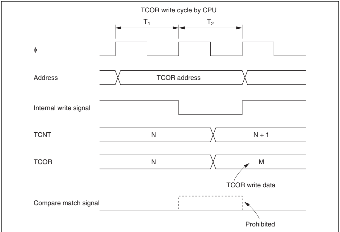
Figure 10.12 Contention between TCOR Write and Compare Match
