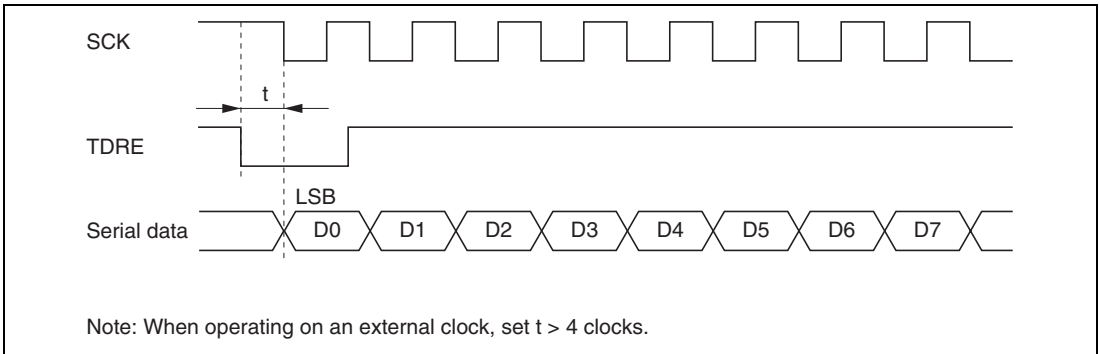
Figure 12.22 Example of Clocked Synchronous Transmission by DTC
