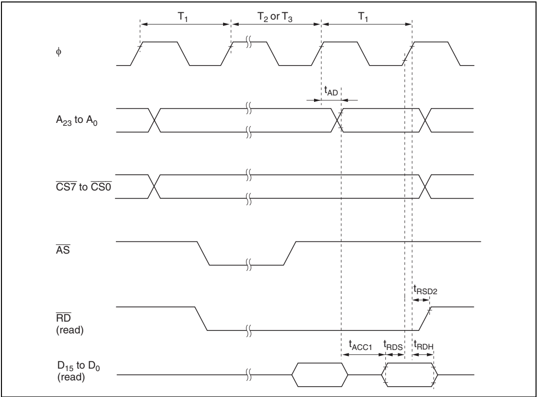
Figure 20.12 Burst ROM Access Timing (One-State Access)
