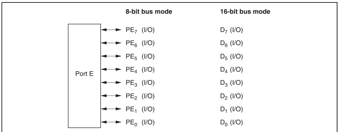
Figure 8.23 Port E Pin Functions (Modes 1, 2, 4, 5, and 6)
