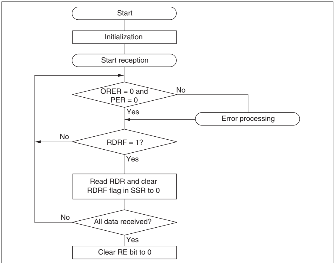
Figure 13.7 Example of Reception Processing Flow
