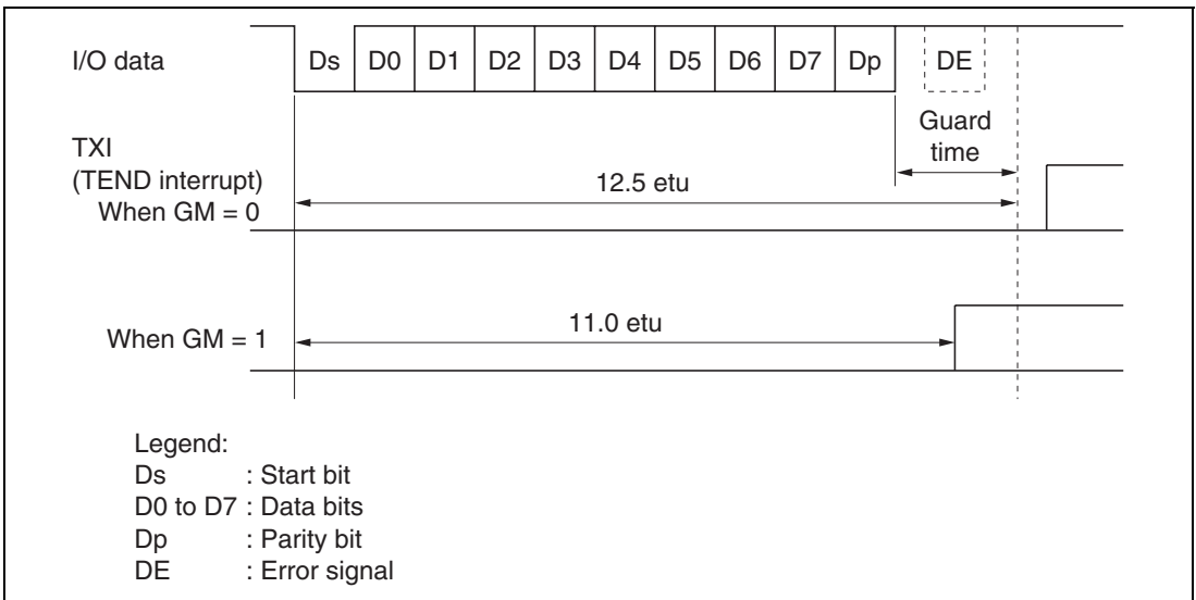
Figure 13.6 TEND Flag Generation Timing in Transmission Operation
