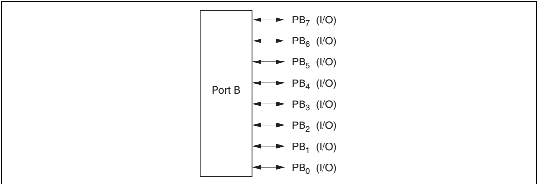
Figure 8.14 Port B Pin Functions (Modes 3 and 7)
