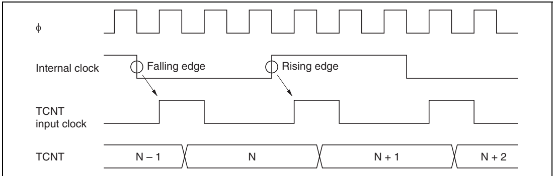
Figure 9.34 Count Timing in Internal Clock Operation
