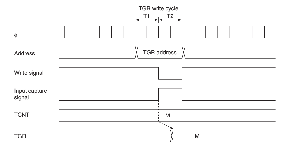
Figure 9.54 Contention between TGR Write and Input Capture
