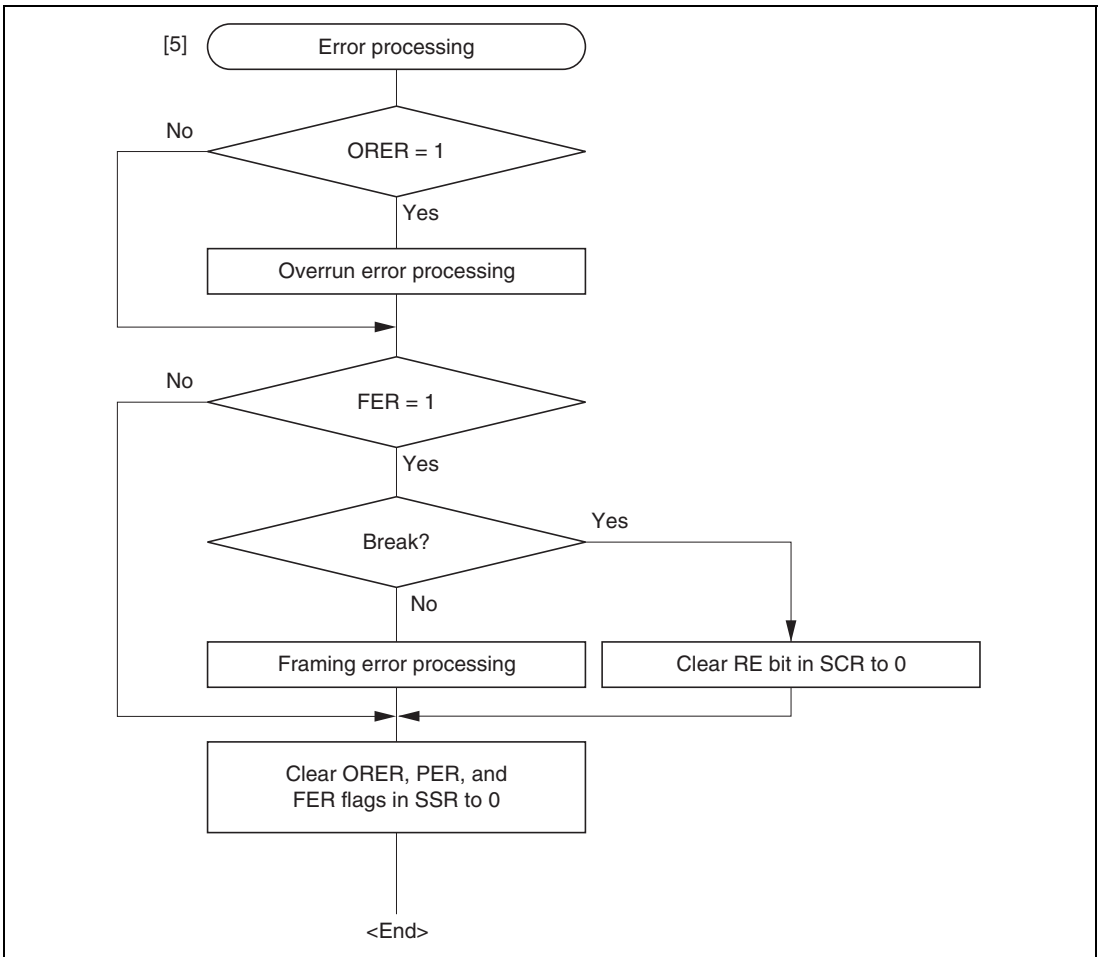
Figure 12.12 Sample Multiprocessor Serial Reception Flowchart (cont)
