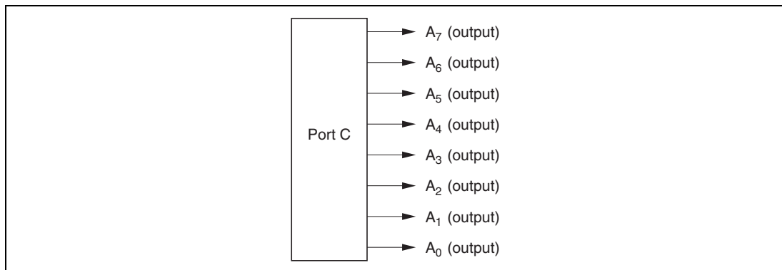
Figure 8.16 Port C Pin Functions (Modes 1, 4, and 5)
