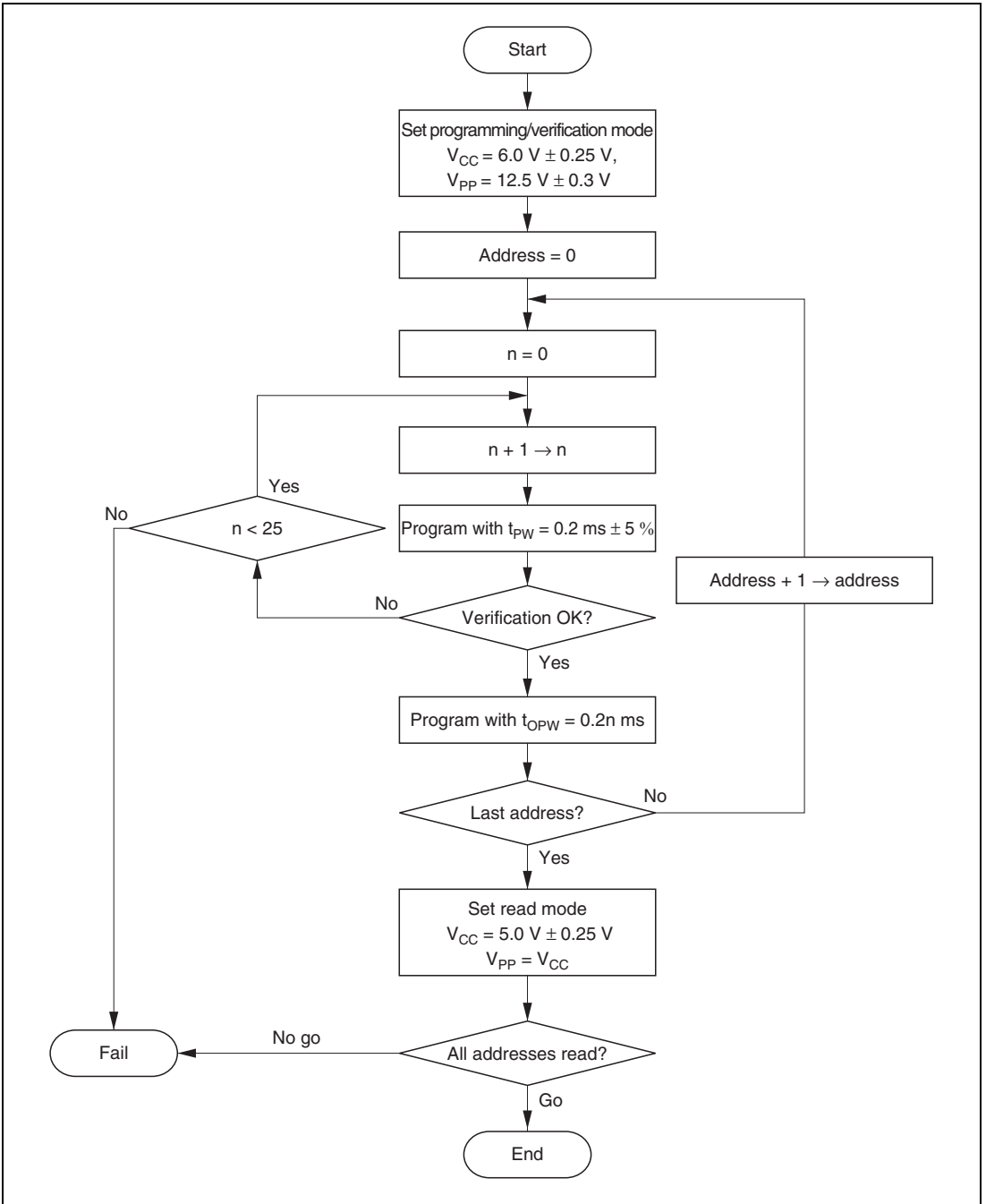
Figure 17.4 High-Speed Programming Flowchart
