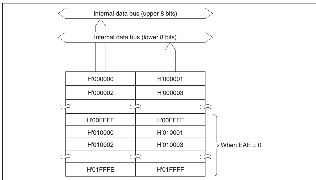
Figure 17.1 Block Diagram of ROM (H8S/2355)
