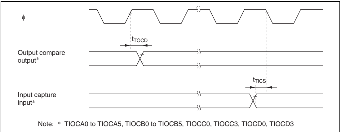
Figure 20.15 TPU Input/Output Timing
