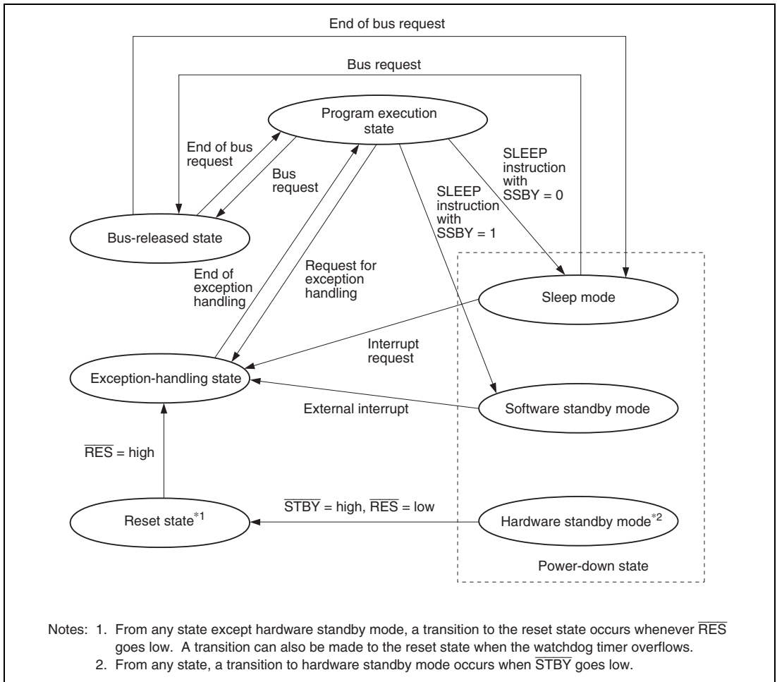
Figure 2.15 State Transitions
