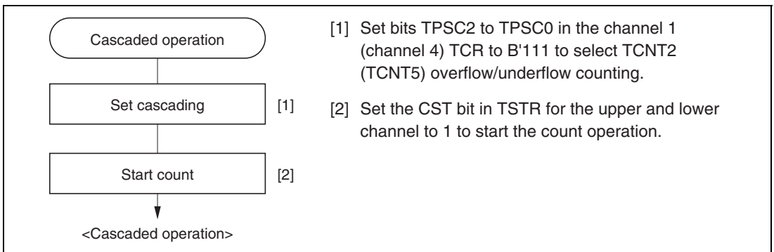
Figure 9.21 Cascaded Operation Setting Procedure
