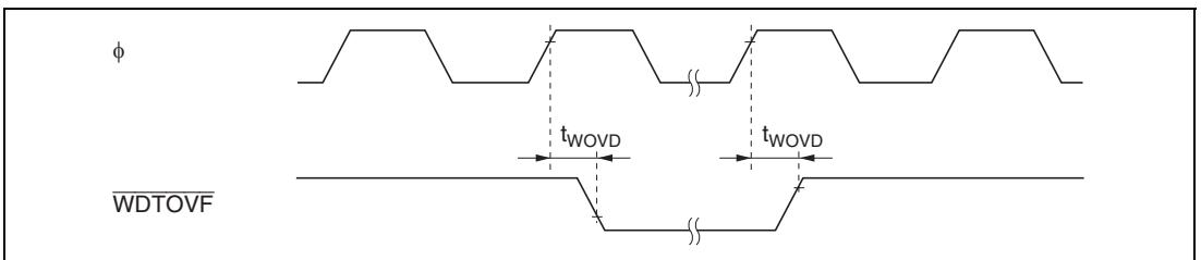
Figure 20.20 WDT Output Timing
