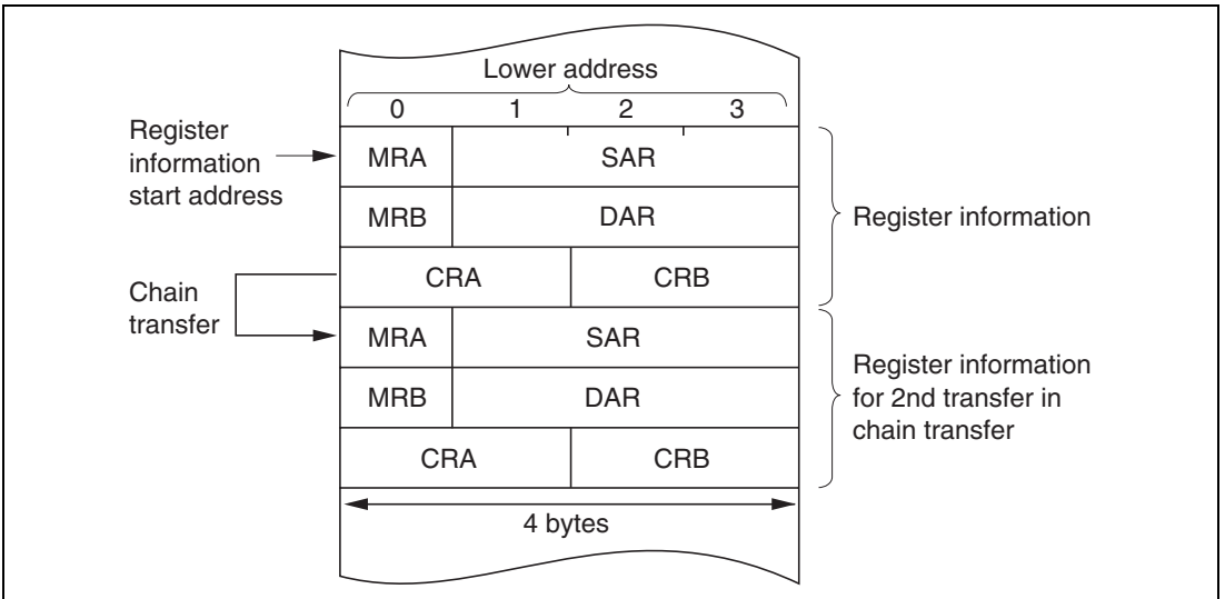
Figure 7.5 Location of Register Information in Address Space
