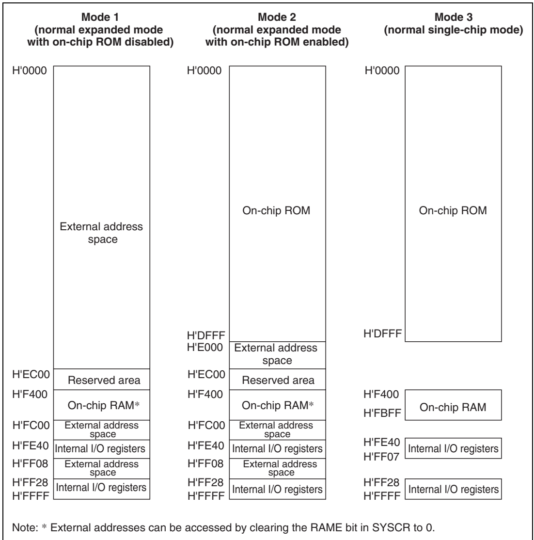
Figure 3.2 Memory Map in Each Operating Mode in the H8S/2353
