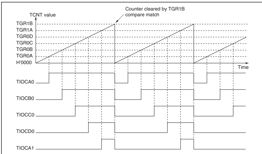
Figure 9.26 Example of PWM Mode Operation (2)
