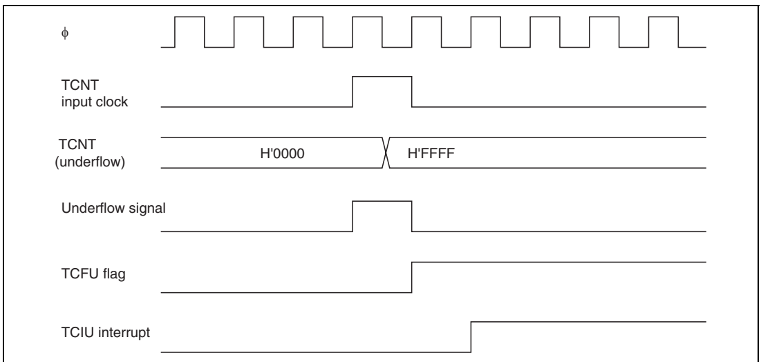
Figure 9.45 TCIU Interrupt Setting Timing
