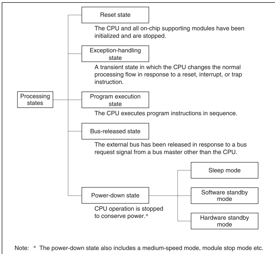
Figure 2.14 Processing States
