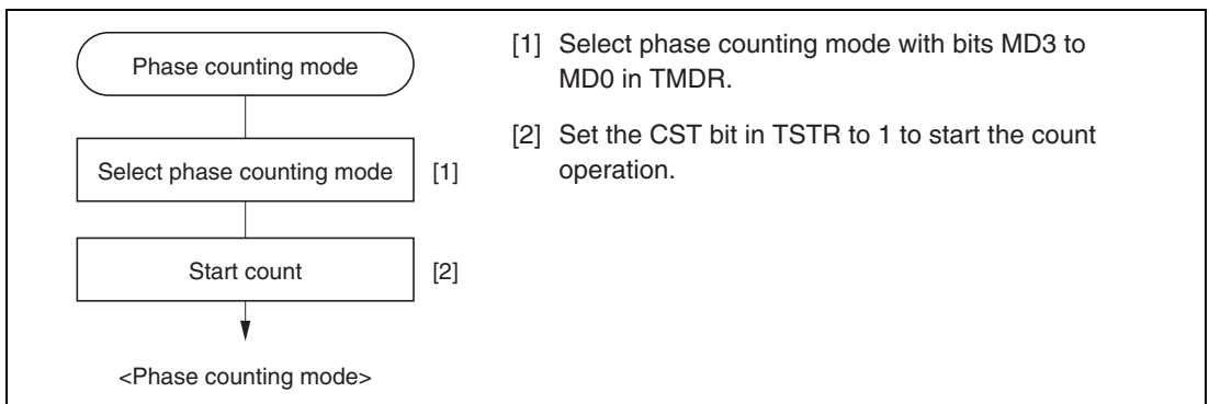
Figure 9.28 Example of Phase Counting Mode Setting Procedure
