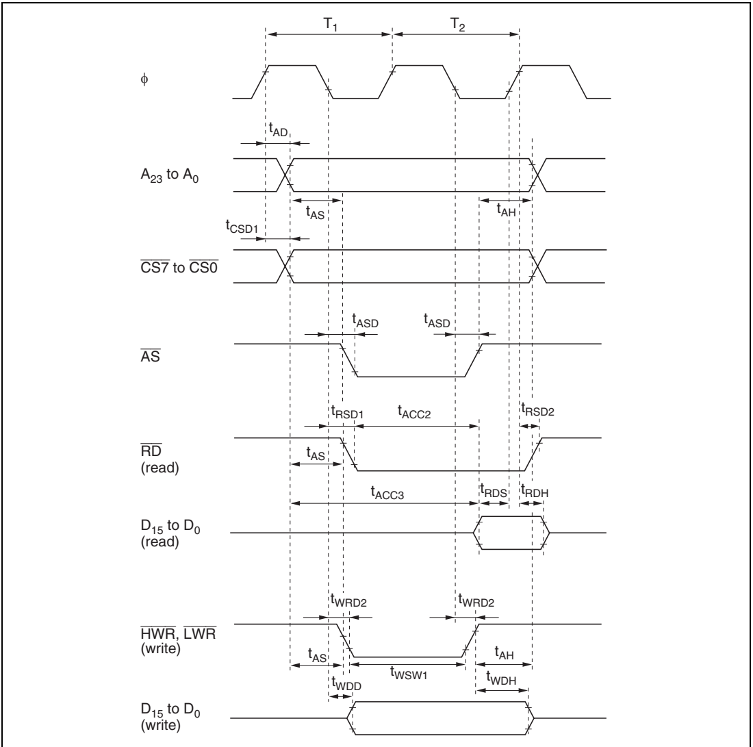
Figure 20.8 Basic Bus Timing (Two-State Access)
