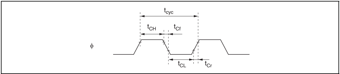
Figure 20.4 System Clock Timing
