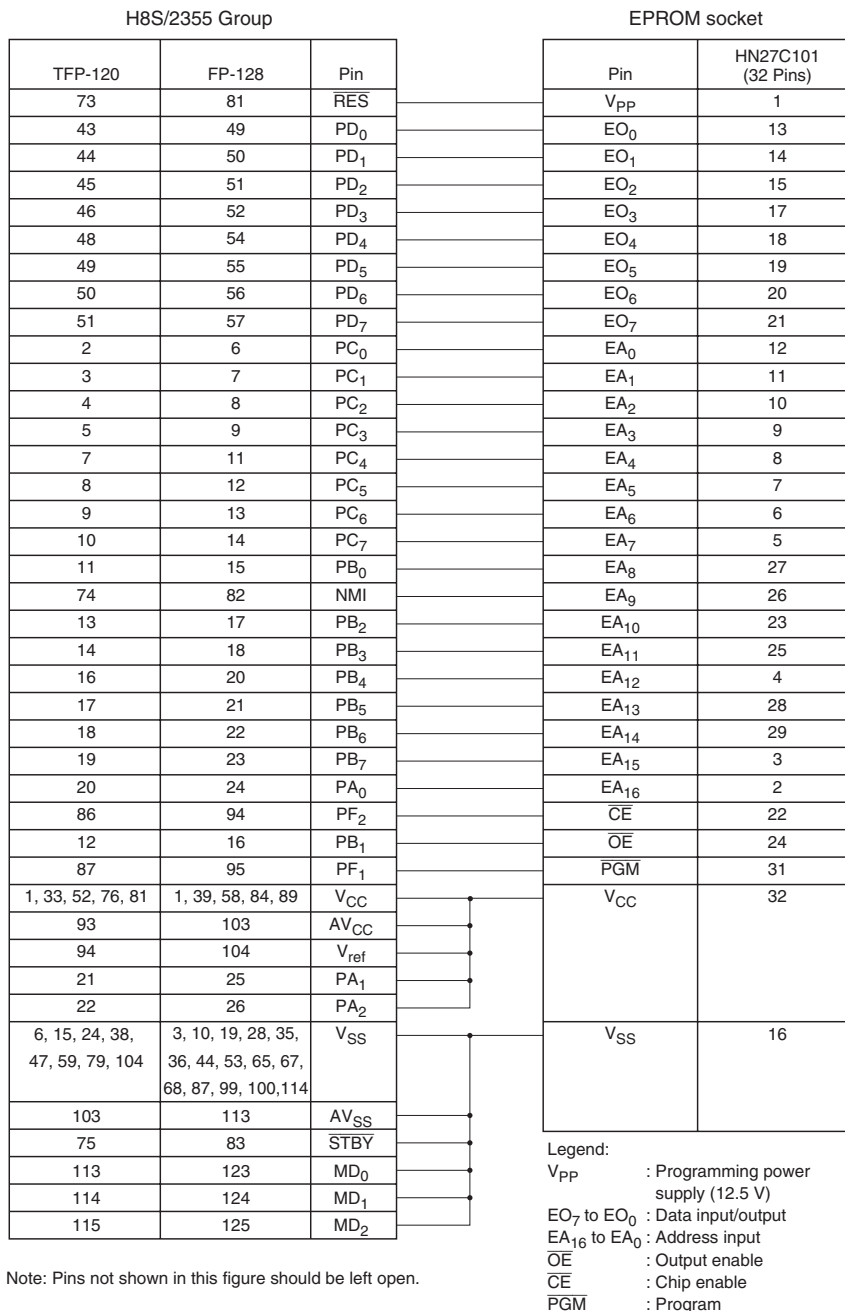
Figure 17.2 Wiring of 120-Pin/32-Pin Socket Adapter
