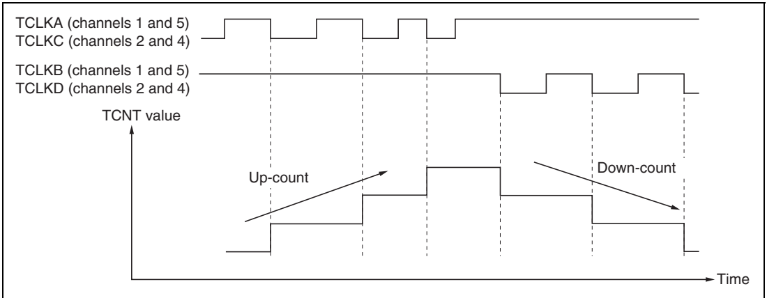
Figure 9.31 Example of Phase Counting Mode 3 Operation
