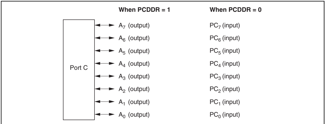
Figure 8.17 Port C Pin Functions (Modes 2 and 6)
