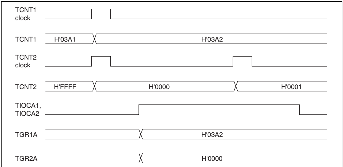
Figure 9.22 Example of Cascaded Operation (1)
