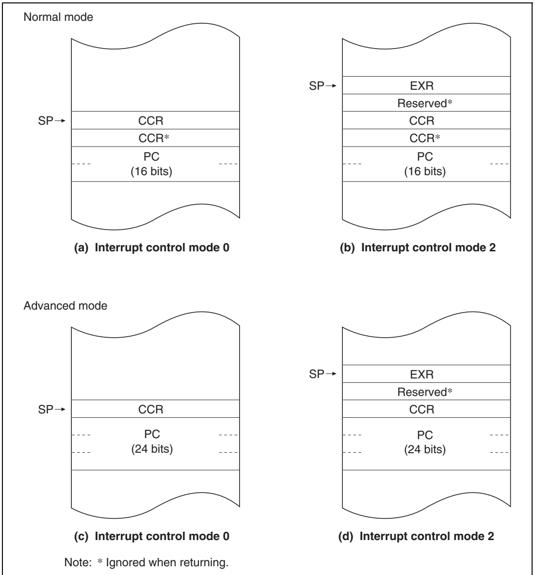
Figure 2.16 Stack Structure after Exception Handling (Examples)
