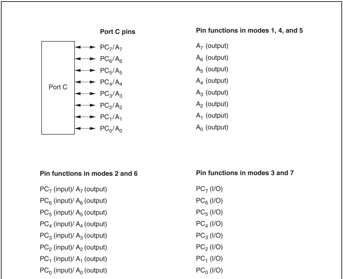
Figure 8.15 Port C Pin Functions
