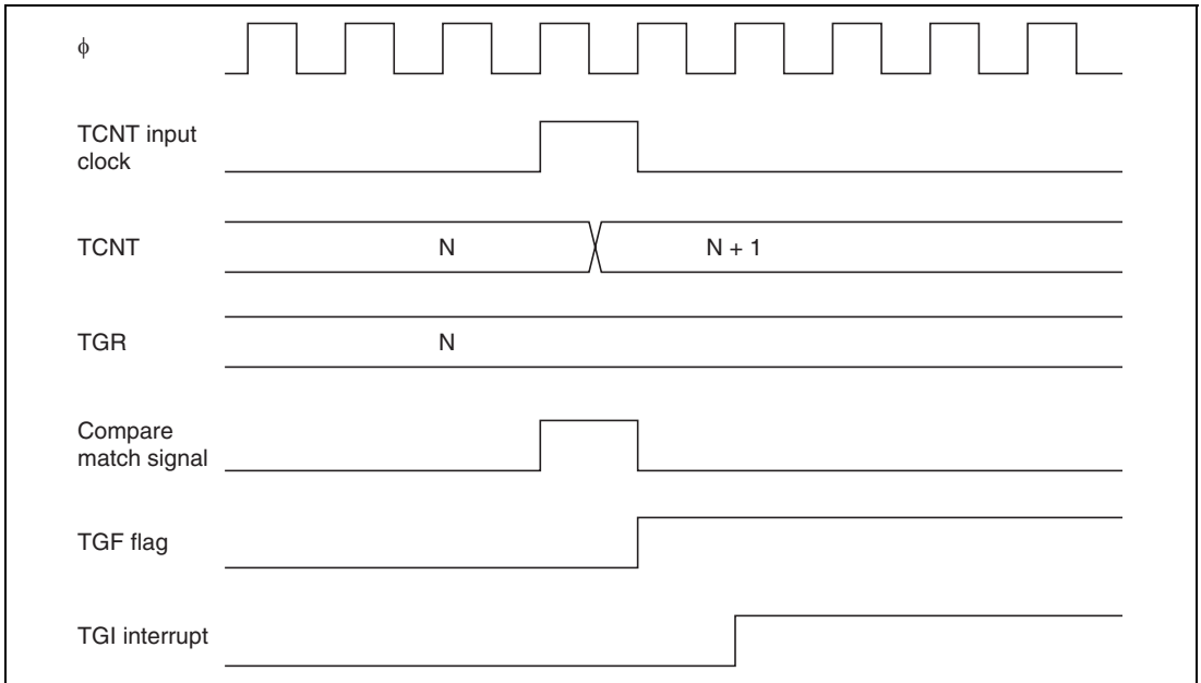
Figure 9.42 TGI Interrupt Timing (Compare Match)
