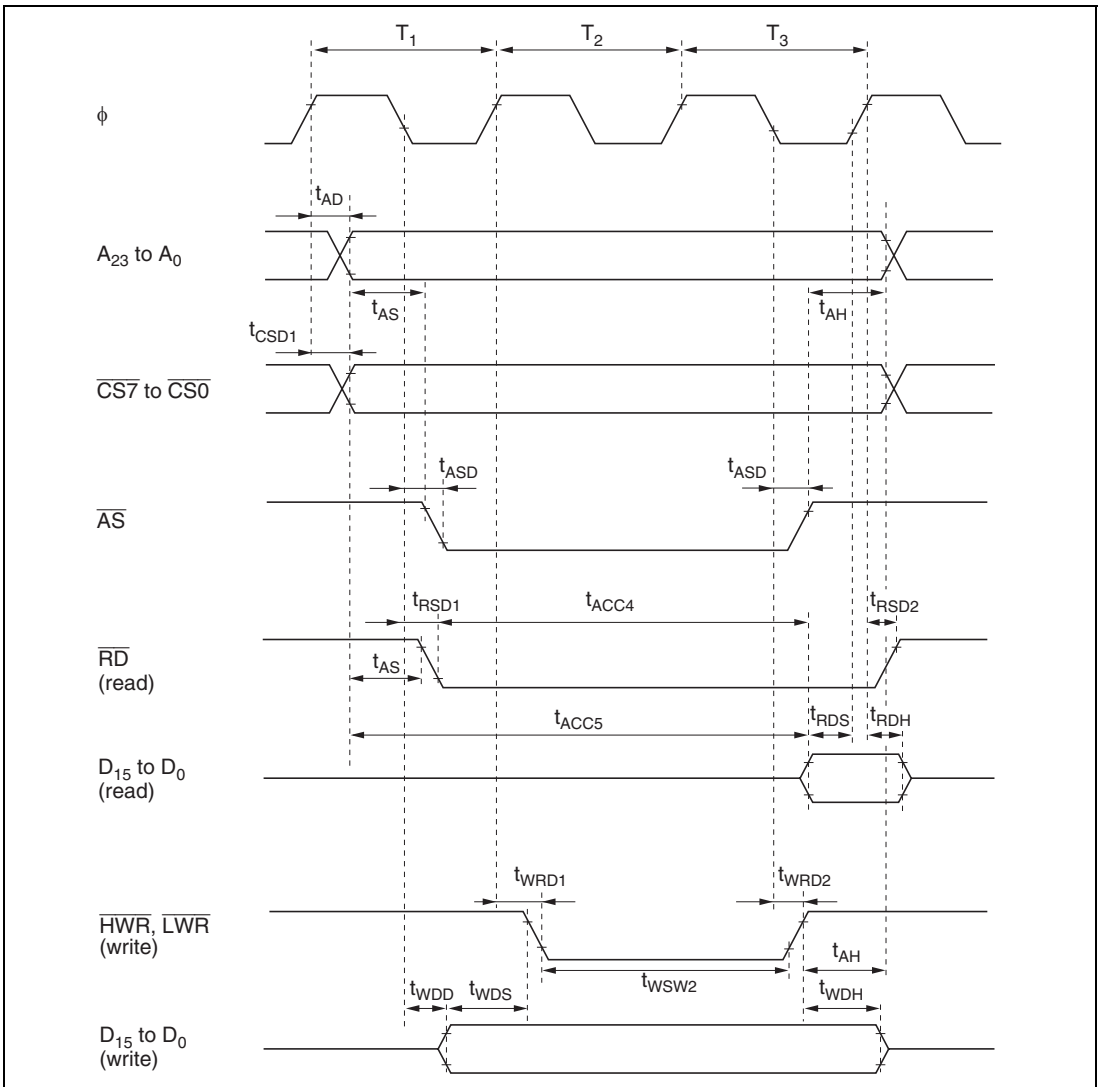
Figure 20.9 Basic Bus Timing (Three-State Access)
