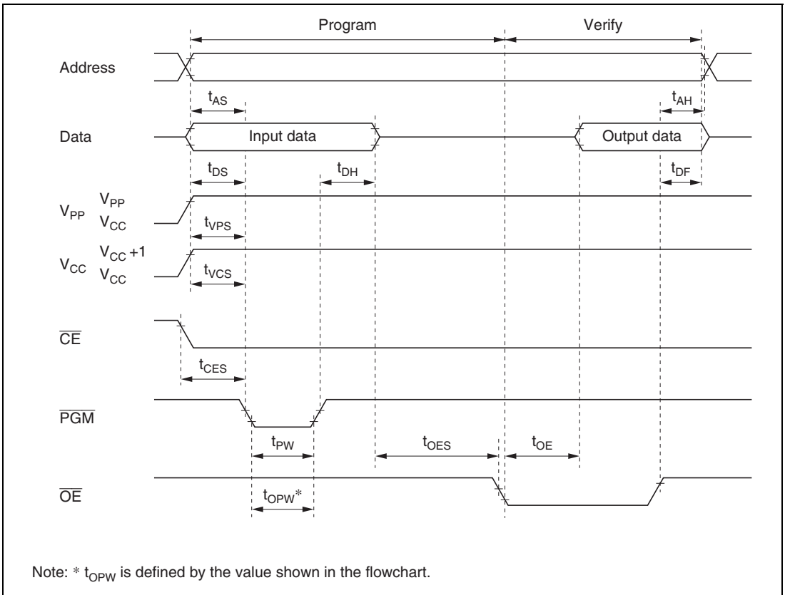
Figure 17.5 PROM Programming/Verification Timing
