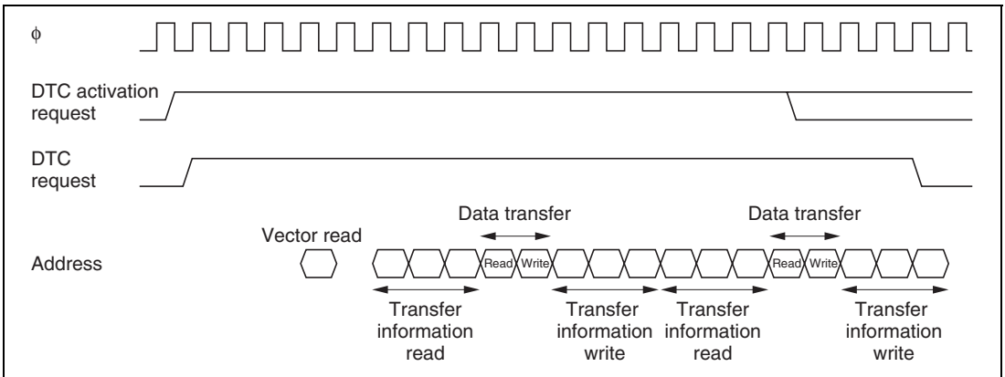
Figure 7.12 DTC Operation Timing (Example of Chain Transfer)
