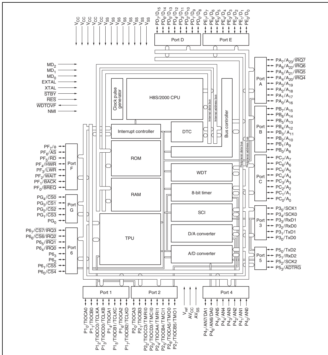
Figure 1.1 Block Diagram (H8S/2355, H8S/2353)
