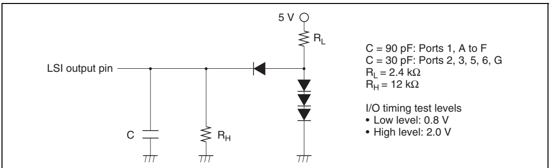
Figure 20.3 Output Load Circuit
