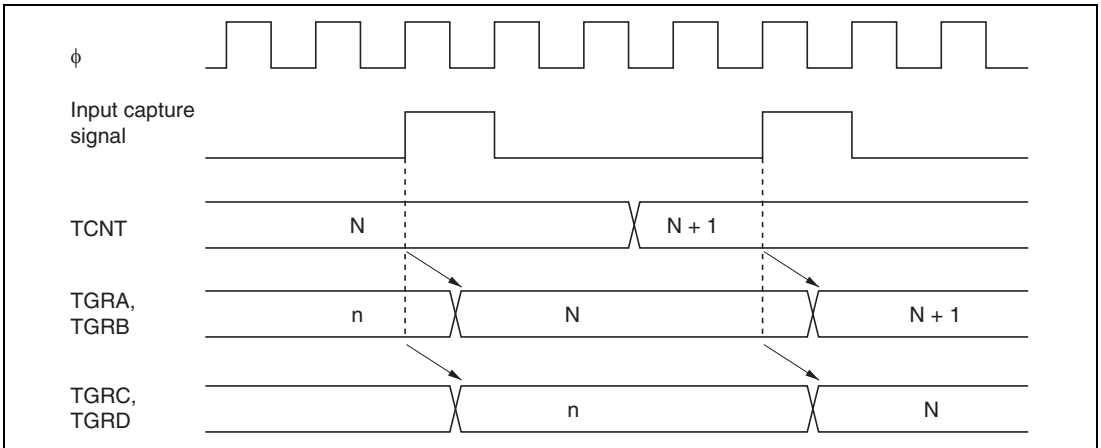
Figure 9.41 Buffer Operation Timing (Input Capture)
