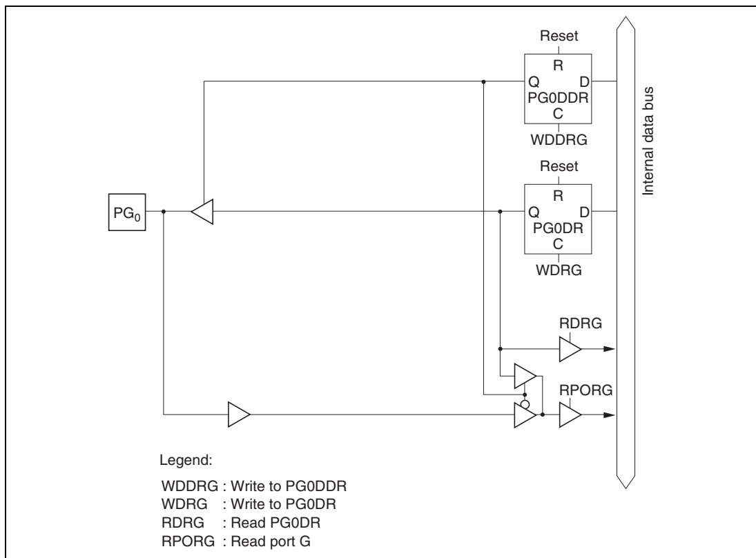
Figure C.13 (a) Port G Block Diagram (Pin PG 0 )
