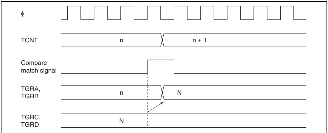
Figure 9.40 Buffer Operation Timing (Compare Match)
