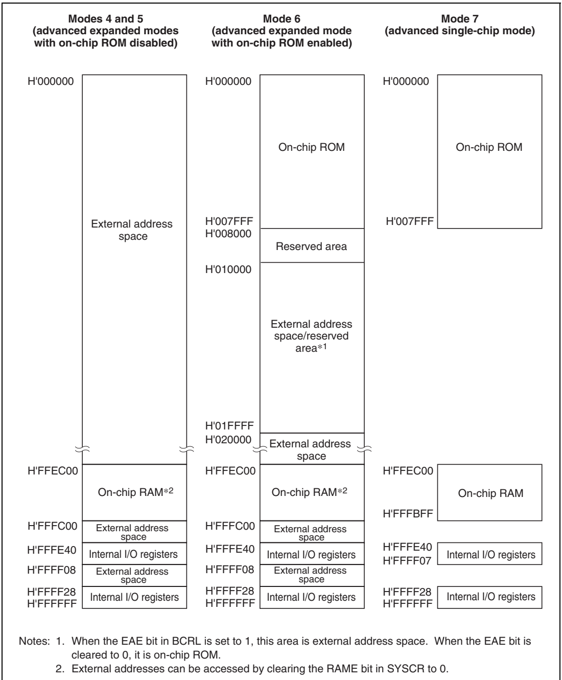
Figure 3.3 Memory Map in Each Operating Mode in the H8S/2393 (cont)
