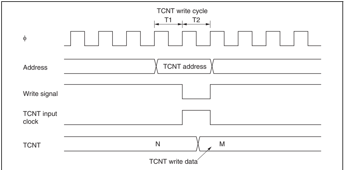
Figure 9.50 Contention between TCNT Write and Increment Operations
