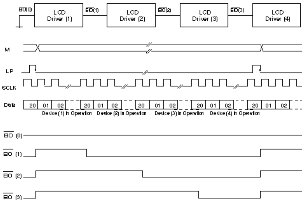
Figure 10. \overline{\text{EIO}}1 and \overline{\text{EIO}}2 in 4 Data Bit Application and Timing Diagram
