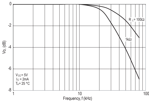
Figure 19. Frequency Response
