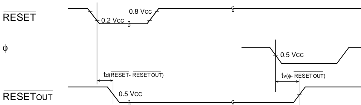
Fig. 3.1.4 Timing diagram (in memory expansion mode and microprocessor mode) (1)
