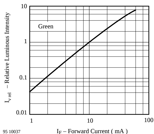
Figure 22. Relative Luminous Intensity vs. Forward Current
