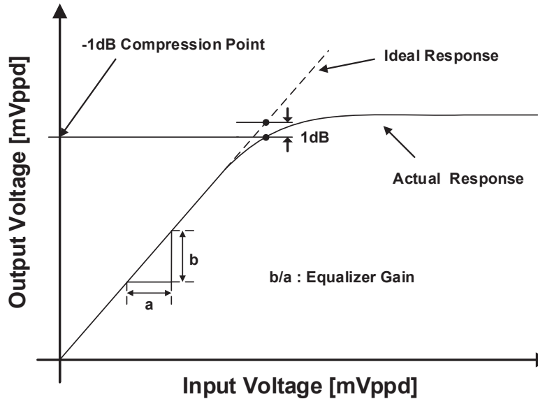
Figure 1. -1dB Compression Point
