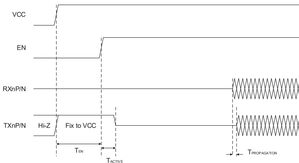
Figure 4. Power on Sequence (SignalDetect Disable/ RxDetect Disable)
