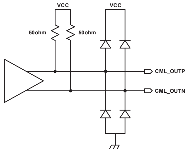
Figure 3. CML Output Schematic Diagram
