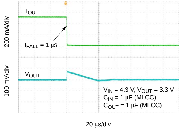
Figure 44. Load Transient Response – 450 mA to 1 mA – V_{OUT} = 3.3 V
