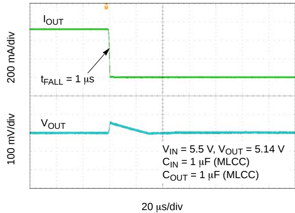
Figure 46. Load Transient Response – 450 mA to 1 mA – V_{OUT} = 5.14 V
