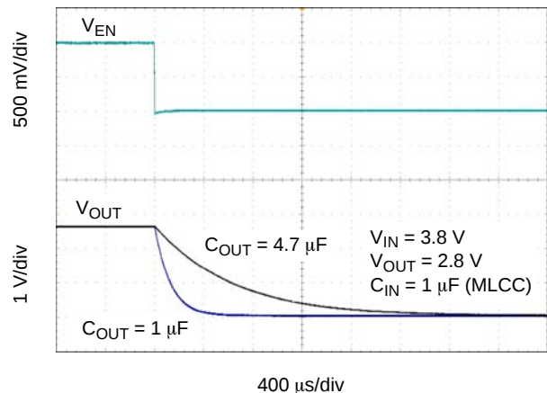
Figure 48. Enable Turn-off
