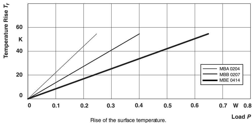
Temperature Rise
