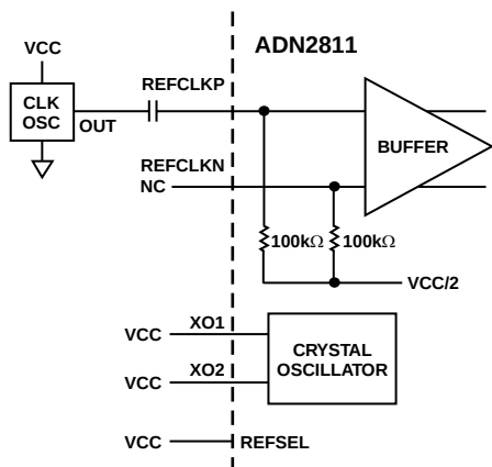
Figure 15. Single-Ended REFCLK Configuration
