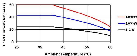
Derating Curve: DC60A60
