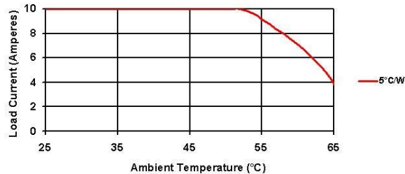
Derating Curve: DC60A10
