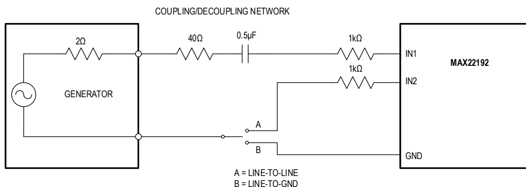
Figure 19. Surge Testing Methods
