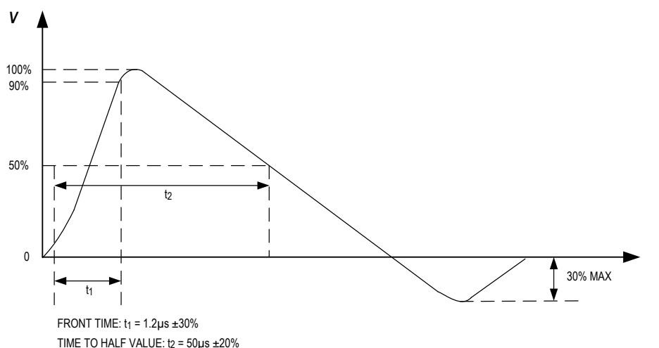
Figure 18. 1.2/50μs Surge Voltage Waveform
