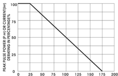
FIGURE 2-DERATING CURVE
