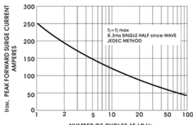
FIG. 6-MAXIMUM NON-REPETITIVE PEAK FORWARD SURGE CURRENT UNIDIRECTIONAL
