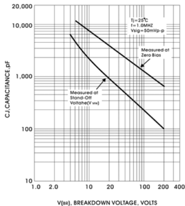
FIGURE 4-TYPICAL CAPACITANCE VS STAND-OFF VOLTAGE
