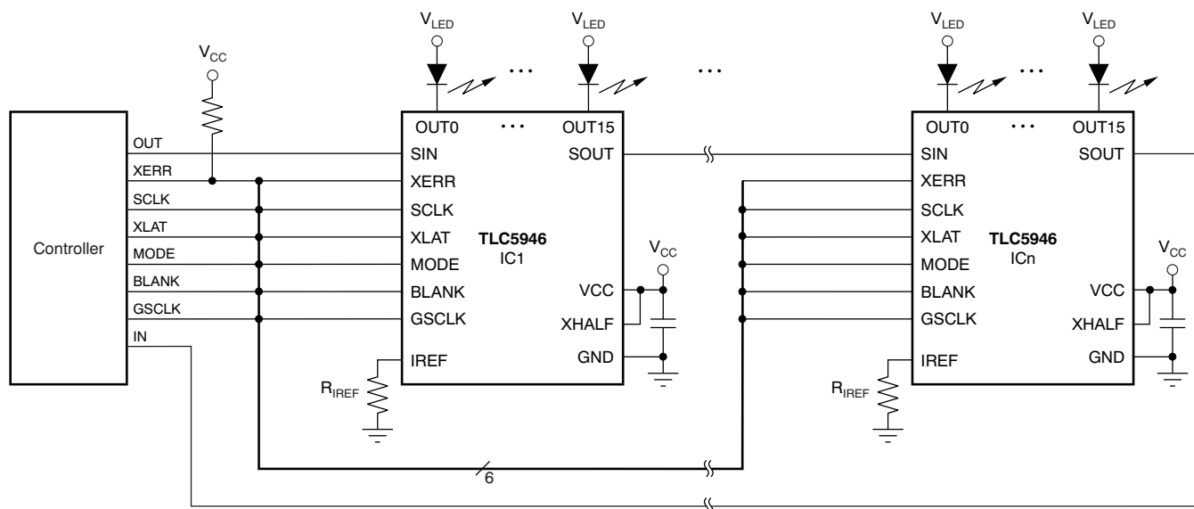
Figure 32. Cascading Device Connections
