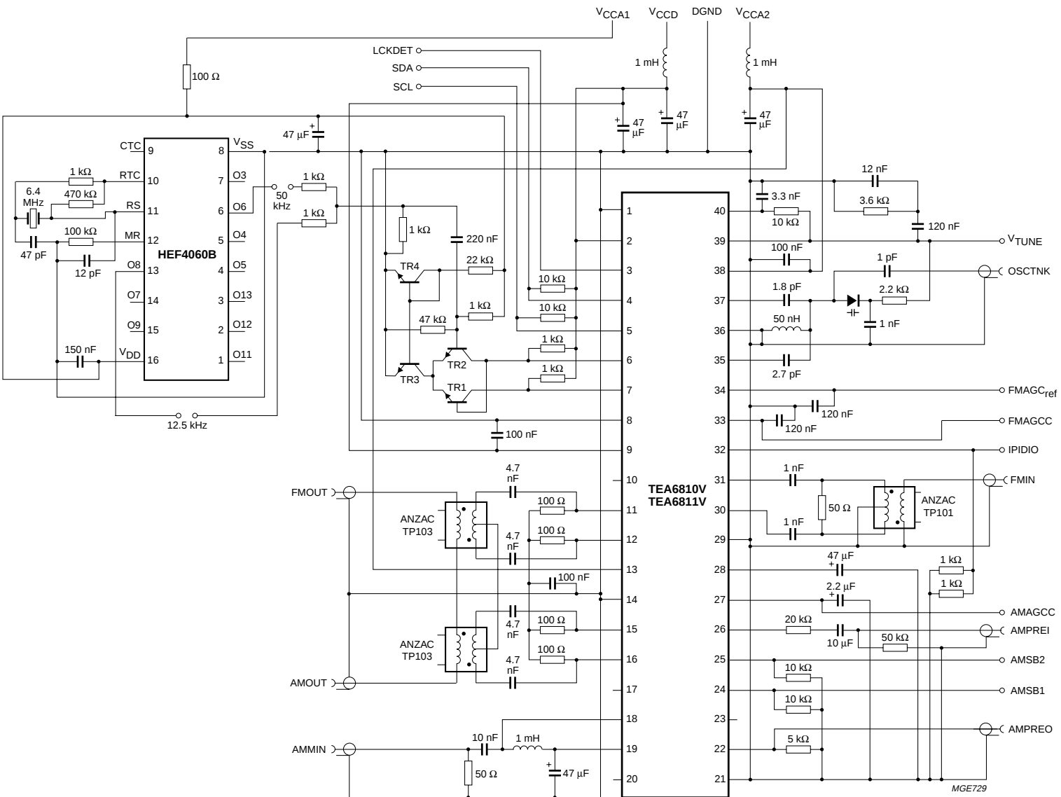
Fig.8 Test board diagram.
