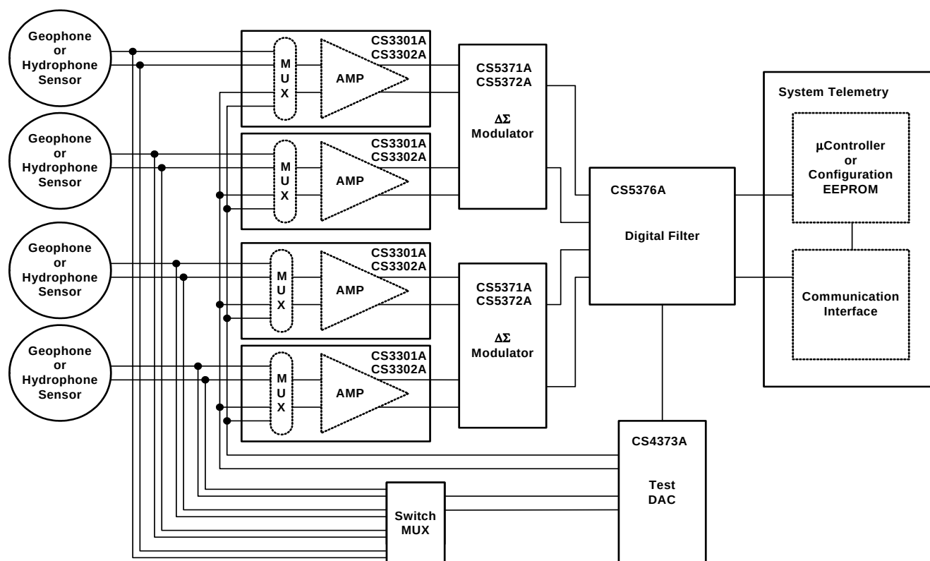
Figure 3. System Architecture
