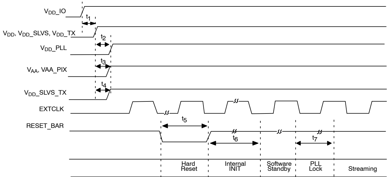
Figure 45. Power-Up Sequence
