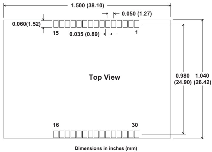
DNT24MCA Solder Pad Dimensions
