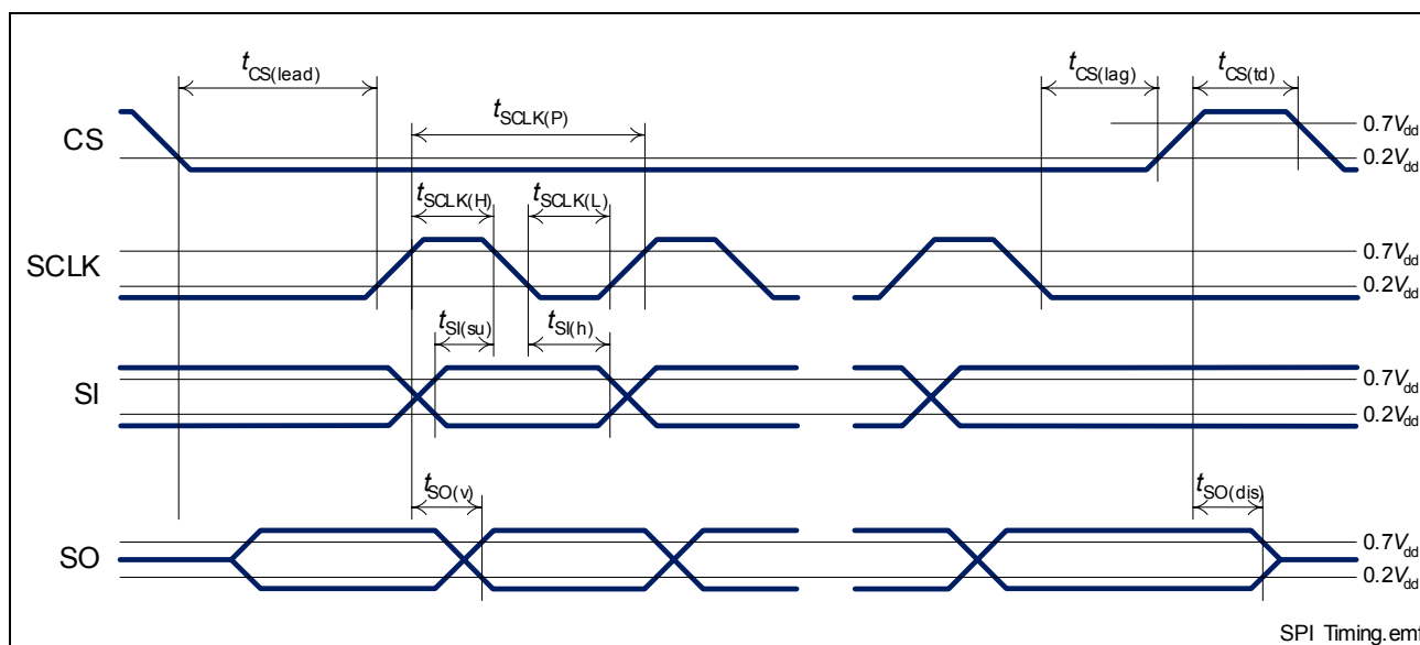
Figure 13 Timing Diagram
