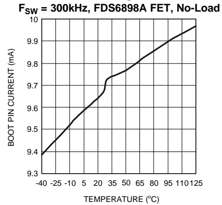
BOOT Pin Current vs Temperature for BOOT Voltage = 3.3V
