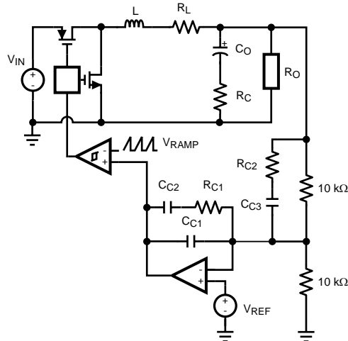
Figure 13. Power Stage and Error Amp
