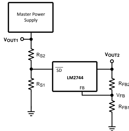
Figure 6. Sequencing Circuit
