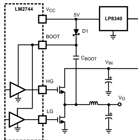
Figure 10. LP8340 Feeding Basic Charge Pump
