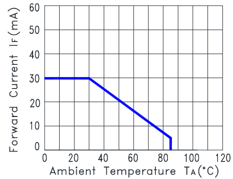
Fig.2 Forward Current Green Derating Curve
