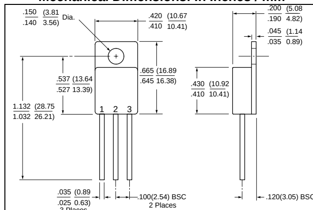
Mechanical Dimensions: In Inches / mm
