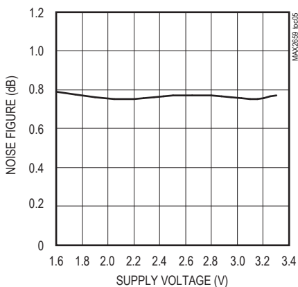
NOISE FIGURE vs. SUPPLY VOLTAGE
