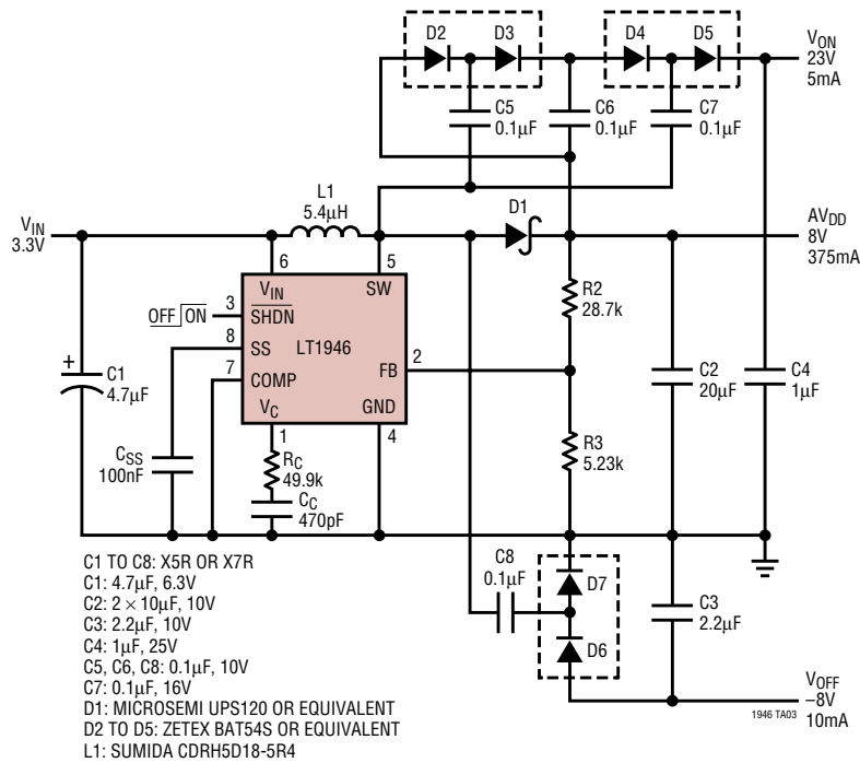
Low Profile, Triple Output TFT Supply (8V, -8V, 23V)
