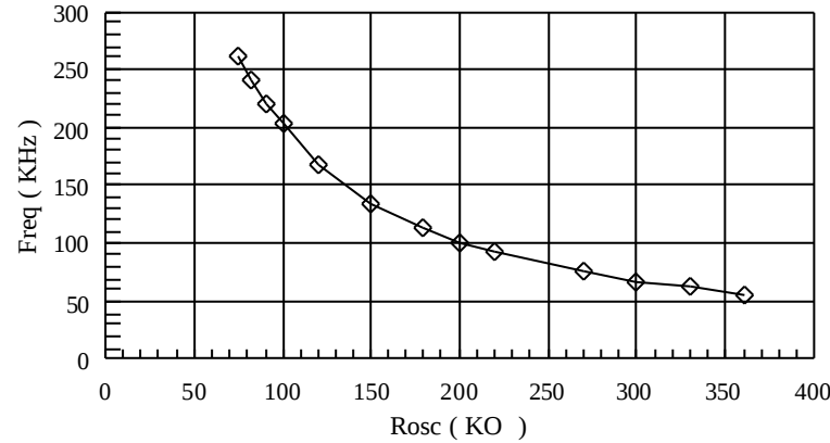
Freq-Rosc Chart ( @Vdd=12V )
