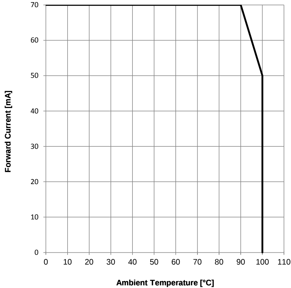
Derating Curve:
