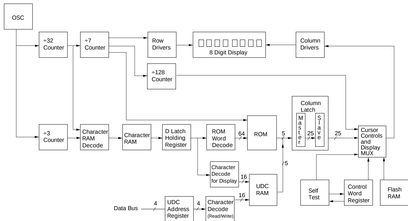
Figure 7. Block diagram
