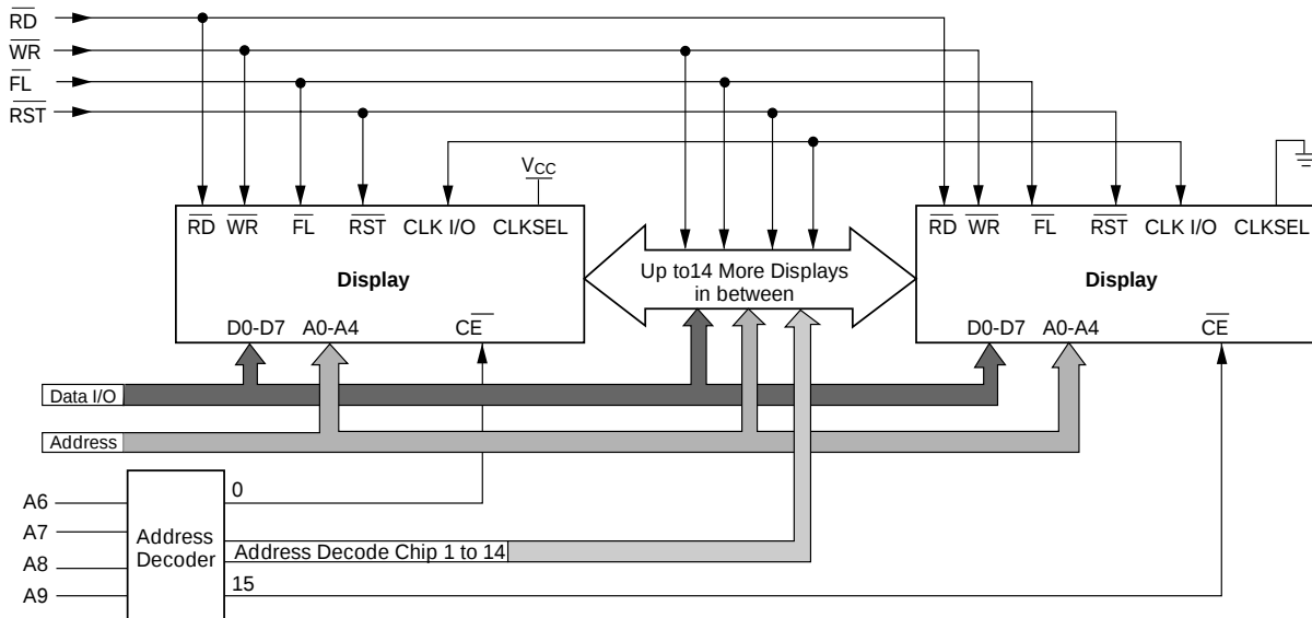
Figure 4. Cascading diagram
